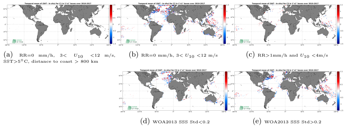
Figure 12: Temporal mean gridded over spatial boxes of size 1^\circ \times 1^\circ of \Delta SSS (SMOS-L3-CATDS-CECOS-IFREMER-V2-1DAY-0.5DEG - TSG-LEGOS-DM) for 5 different subdatasets corresponding to:RR=0 mm/h, 3 < U_{10} < 12 m/s, SST >5^\circ C, distance to coast > 800 km (a), RR=0 mm/h, 3 < U_{10} < 12 m/s (b), RR >1 mm/h and U_{10} < 4 m/s (c), WOA2013 SSS Std <0.2 (d), WOA2013 SSS Std >0.2 (e).
