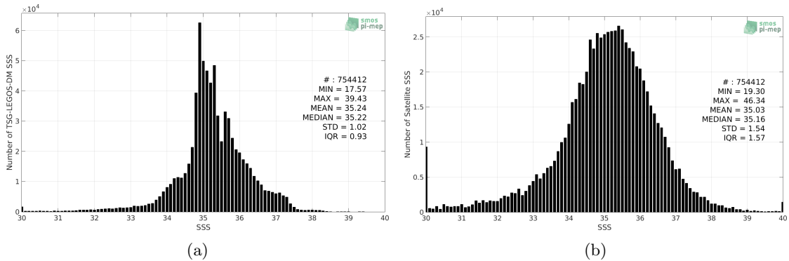
Figure 2: Histograms of SSS from TSG-LEGOS-DM (a) and SMOS-L3-CATDS-CECOS-IFREMER-V2-1DAY-0.5DEG (b) considering all match-up pairs per bins of 0.1 over the SMOS coastal zone ( \approx 800 km) 60N-60S Pi-MEP region and for the full satellite product period.
