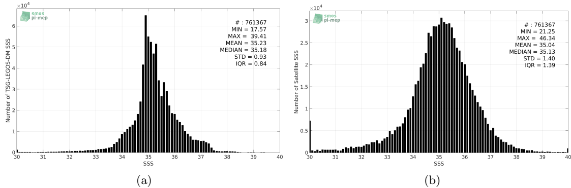
Figure 2: Histograms of SSS from TSG-LEGOS-DM (a) and SMOS-L3-CATDS-CECOS-IFREMER-V2-1DAY-0.5DEG (b) considering all match-up pairs per bins of 0.1 over the SMOS coastal zone ( \approx 800\text{km} ) 60N-60S Pi-MEP region and for the full satellite product period.
