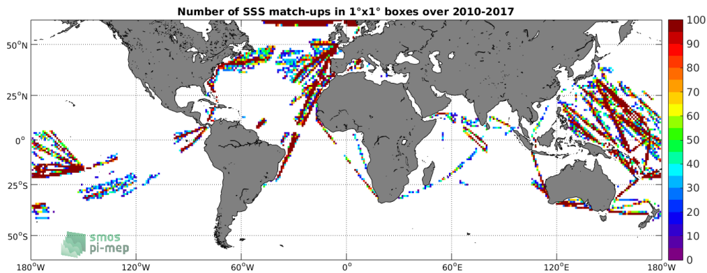
Figure 4: Number of SSS match-ups between TSG-LEGOS-DM SSS and the SMOS-L3-CATDS-CECOS-IFREMER-V2-1DAY-0.5DEG SSS product for the SMOS coastal zone ( \pm 800\text{km} ) 60N-60S Pi-MEP region over 1^\circ \times 1^\circ boxes and for the full satellite product period.
