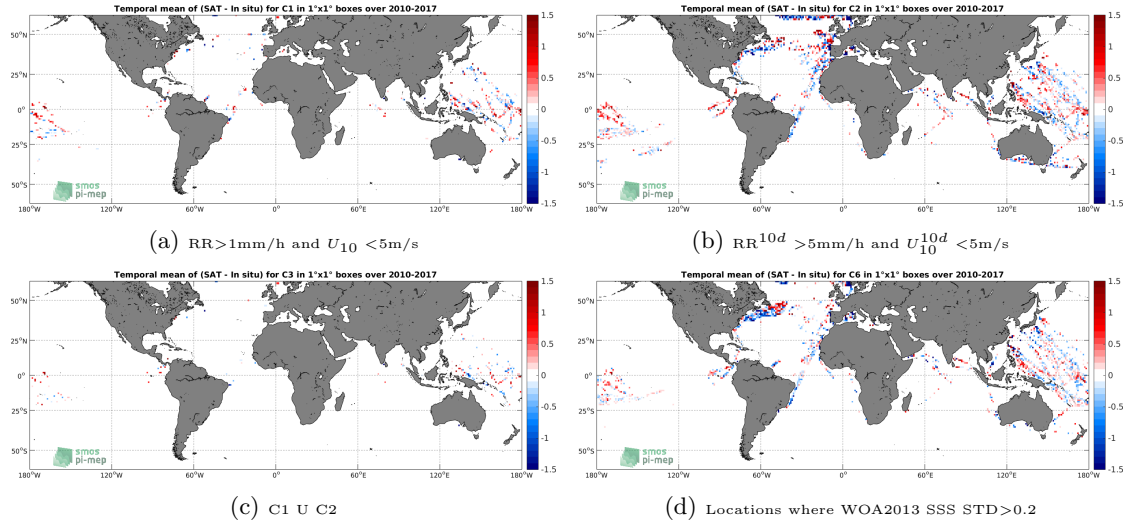
Figure 12: Temporal mean gridded over spatial boxes of size 1^\circ \times 1^\circ of \Delta SSS (SMOS-L3-CATDS-CECOS-IFREMER-V2-1DAY-0.5DEG - TSG-LEGOS-DM) for 4 different subdatasets corresponding to: RR > 1\text{mm/h} and U_{10} < 5\text{m/s} (a), RR^{10d} > 5\text{mm/h} and U_{10}^{10d} < 5\text{m/s} (b), C1 U C2 (c), Locations where WOA2013 SSS STD > 0.2 (d).
