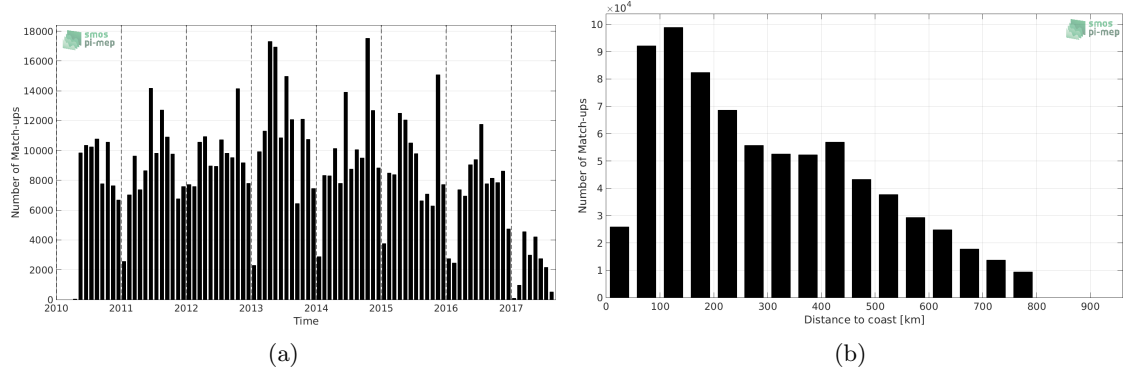
Figure 1: Number of match-ups between TSG-LEGOS-DM and SMOS-L3-CATDS-CECOS-IFREMER-V2-1DAY-0.5DEG SSS as a function of time (a) and as function of the distance to coast (b) over the SMOS coastal zone ( \approx 800\text{km} ) 60N-60S Pi-MEP region and for the full satellite product period.
