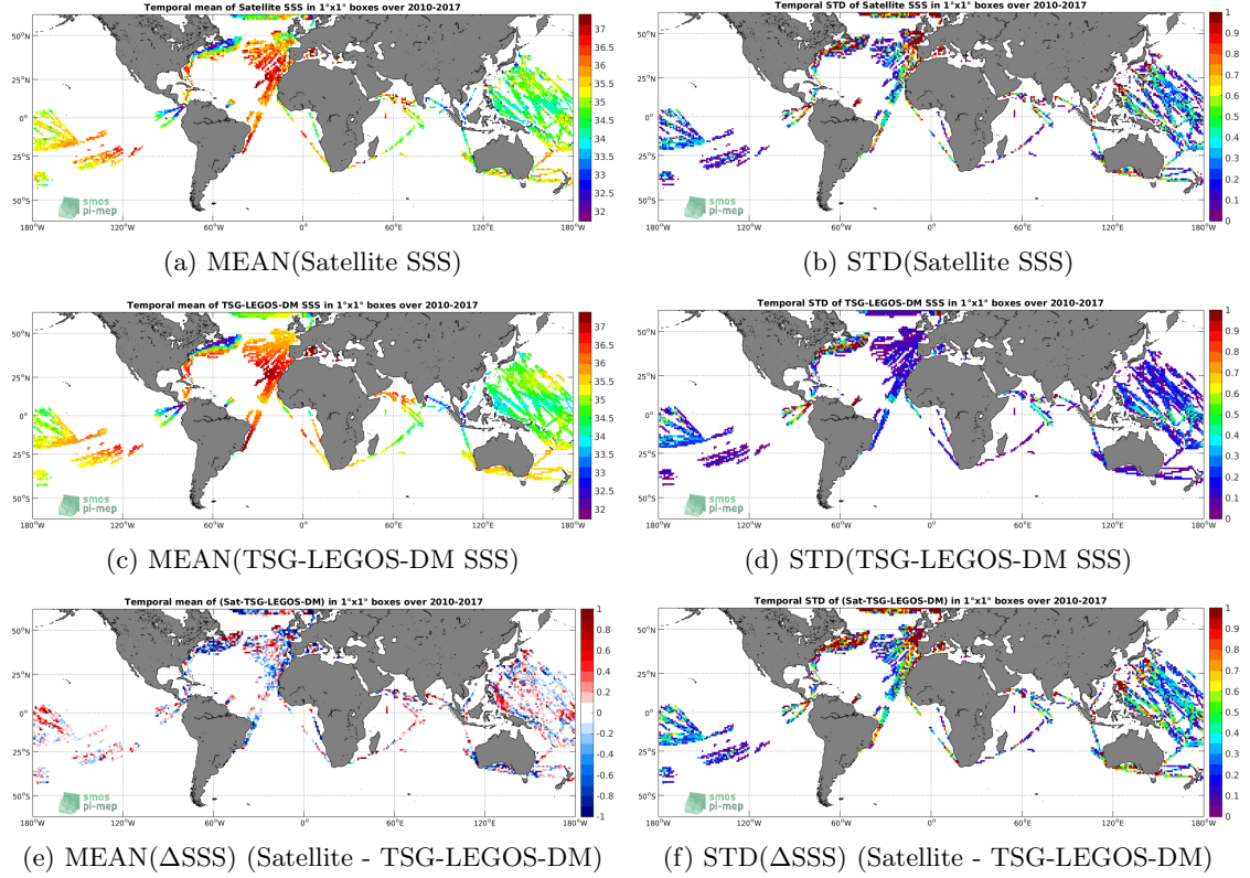
Figure 6: Temporal mean (left) and STD (right) of SSS from SMOS-L3-CATDS-CECOS-IFREMER-V2-1DAY-0.5DEG (top), TSG-LEGOS-DM (middle), and of \Delta SSS (Satellite - TSG-LEGOS-DM). Only match-up pairs are used to generate these maps.
