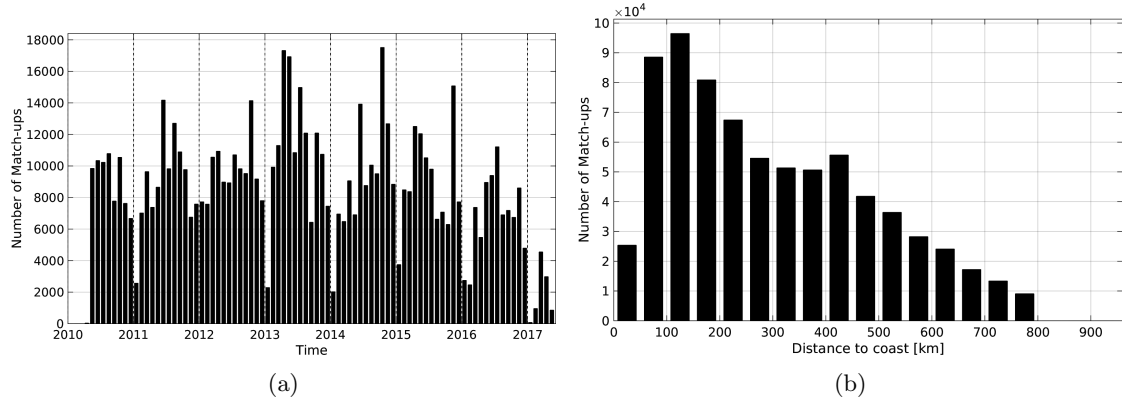
Figure 1: Number of match-ups between TSG-LEGOS-DM and SMOS-L3-CATDS-CECOS-IFREMER-V2-1DAY-0.5DEG SSS as a function of time (a) and as function of the distance to coast (b) over the SMOS coastal zone ( \pm 800\text{km} ) 60N-60S Pi-MEP region and for the full satellite product period.
