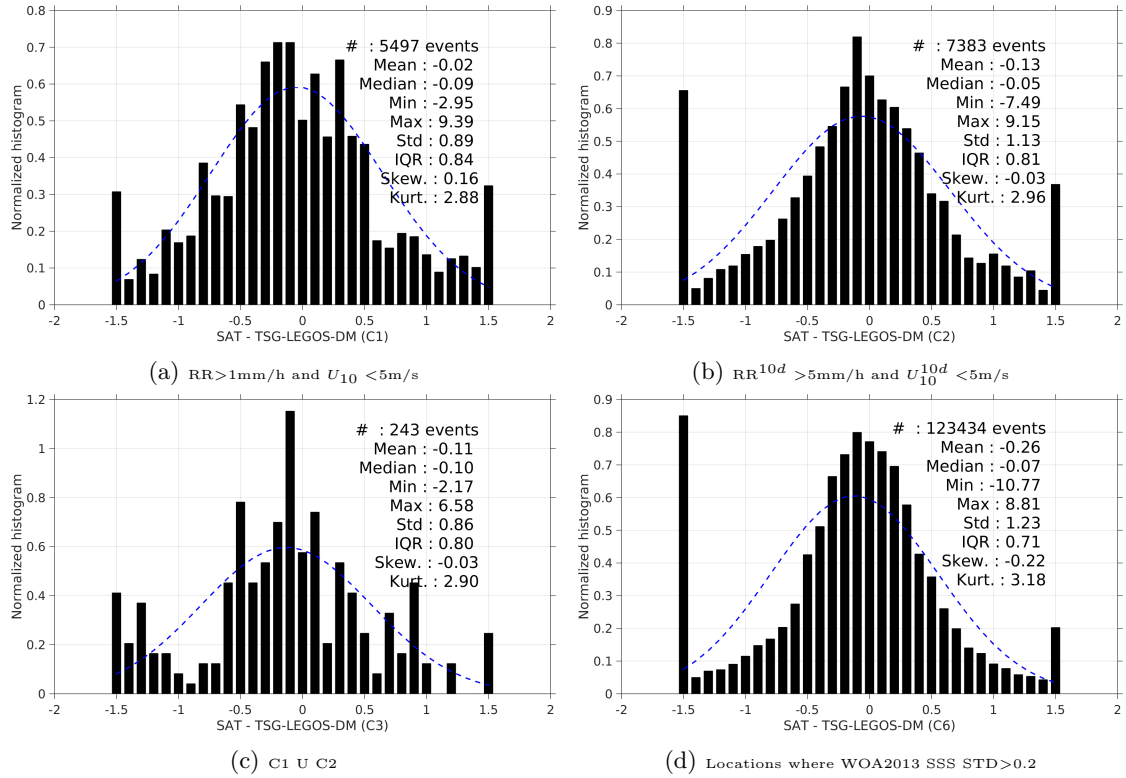
Figure 13: Normalized histogram of \Delta\text{SSS} (SMOS-L3-CATDS-CECOS-IFREMER-V2-1DAY-0.5deg - TSG-LEGOS-DM) for 6 different subdatasets corresponding to: RR > 1mm/h and U_{10} < 5\text{m/s} (a), \text{RR}^{10d} > 5\text{mm/h} and U_{10}^{10d} < 5\text{m/s} (b), C1 U C2 (c), Locations where WOA2013 SSS STD > 0.2 (d).
