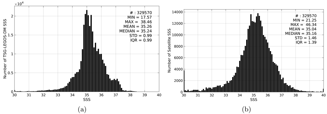
Figure 2: Histograms of SSS from TSG-LEGOS-DM (a) and SMOS-L3-CATDS-CECOS-IFREMER-V2-1DAY-0.5deg (b) considering all match-up pairs per bins of 0.1 over the SMOS coastal zone ( \pm 800\text{km} ) 60N-60S Pi-MEP region and for the full satellite product period.
