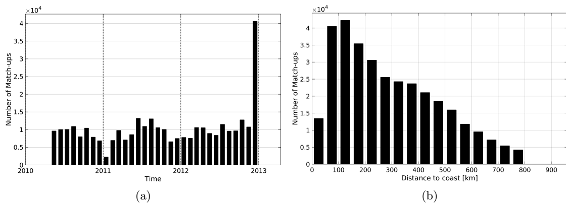
Figure 1: Number of match-ups between TSG-LEGOS-DM and SMOS-L3-CATDS-CECOS-IFREMER-V2-1DAY-0.5deg SSS as a function of time (a) and as function of the distance to coast (b) over the SMOS coastal zone ( \leq 800 km) 60N-60S Pi-MEP region and for the full satellite product period.
