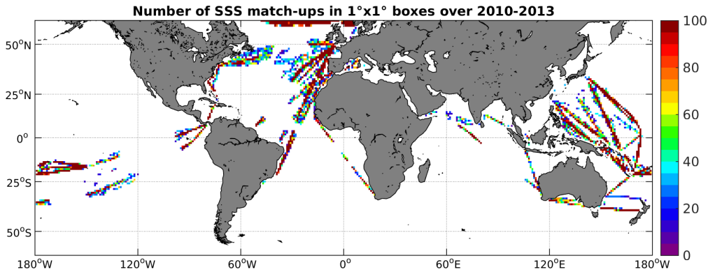
Figure 4: Number of SSS match-ups between TSG-LEGOS-DM SSS and the SMOS-L3-CATDS-CECOS-IFREMER-V2-1DAY-0.5deg SSS product for the SMOS coastal zone ( \approx 800\text{km} ) 60N-60S Pi-MEP region over 1^\circ \times 1^\circ boxes and for the full satellite product period.
