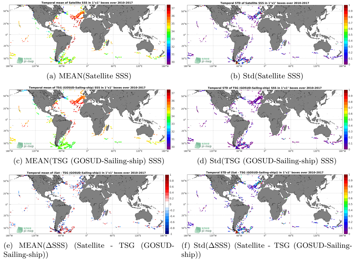
Figure 6: Temporal mean (left) and Std (right) of SSS from SMOS SSS L3 v2 - Daily - 0.5 Deg (CATDS-CECOS-IFREMER) (top), TSG (GOSUD-Sailing-ship) (middle), and of \Delta SSS (Satellite - TSG (GOSUD-Sailing-ship)). Only match-up pairs are used to generate these maps.
