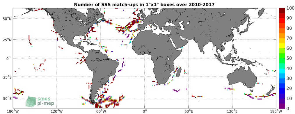
Figure 4: Number of SSS match-ups between TSG (GOSUD-Sailing-ship) SSS and the SMOS SSS L3 v2 - Daily - 0.5 Deg (CATDS-CECOS-IFREMER) SSS product for the SMOS coastal zone (<800km) 60N-60S Pi-MEP region over 1^\circ \times 1^\circ boxes and for the full satellite product period.
