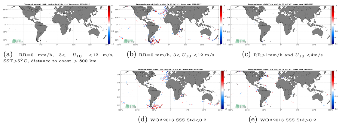
Figure 12: Temporal mean gridded over spatial boxes of size 1^\circ \times 1^\circ of \Delta SSS (SMOS SSS L3 v2 - Daily - 0.5 Deg (CATDS-CECOS-IFREMER) - TSG (GOSUD-Sailing-ship)) for 5 different subdatasets corresponding to: RR=0 mm/h, 3 < U_{10} < 12 m/s, SST > 5°C, distance to coast > 800 km (a), RR=0 mm/h, 3 < U_{10} < 12 m/s (b), RR > 1mm/h and U_{10} < 4 m/s (c), WOA2013 SSS Std < 0.2 (d), WOA2013 SSS Std > 0.2 (e).
