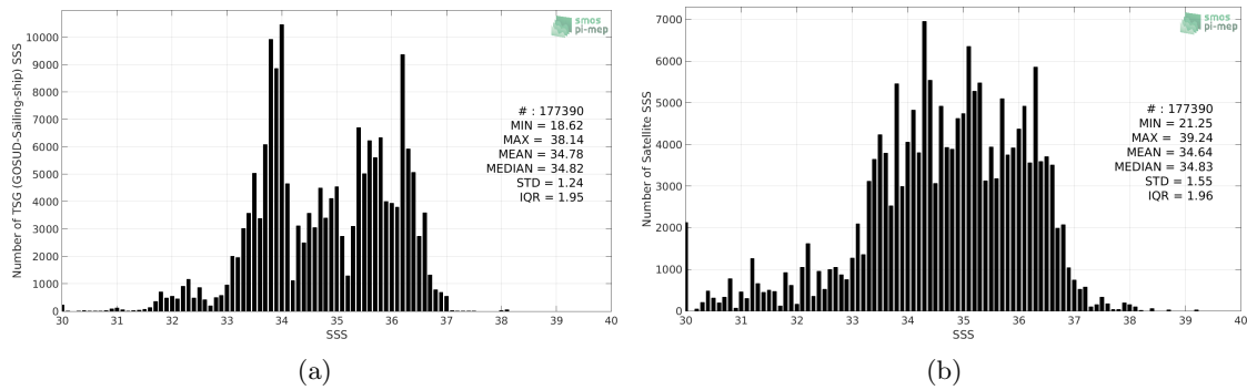
Figure 2: Histograms of SSS from TSG (GOSUD-Sailing-ship) (a) and SMOS SSS L3 v2 - Daily - 0.5 Deg (CATDS-CECOS-IFREMER) (b) considering all match-up pairs per bins of 0.1 over the SMOS coastal zone (<800km) 60N-60S Pi-MEP region and for the full satellite product period.
