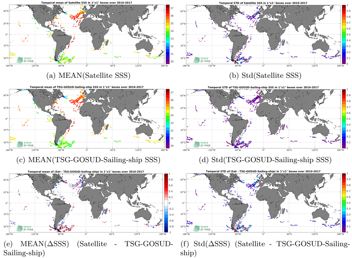
Figure 6: Temporal mean (left) and Std (right) of SSS from SMOS L3 v2 - Daily - 0.5 Deg (CATDS-CECOS-IFREMER) (top), TSG-GOSUD-Sailing-ship (middle), and of \Delta SSS (Satellite - TSG-GOSUD-Sailing-ship). Only match-up pairs are used to generate these maps.
