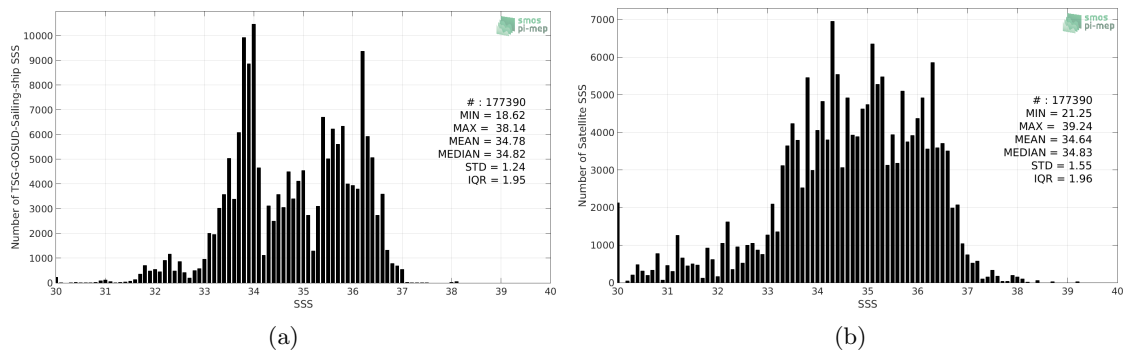
Figure 2: Histograms of SSS from TSG-GOSUD-Sailing-ship (a) and SMOS L3 v2 - Daily - 0.5 Deg (CATDS-CECOS-IFREMER) (b) considering all match-up pairs per bins of 0.1 over the SMOS coastal zone (<800km) 60N-60S Pi-MEP region and for the full satellite product period.
