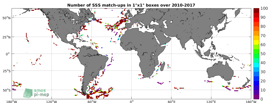
Figure 4: Number of SSS match-ups between TSG-GOSUD-Sailing-ship SSS and the SMOS L3 v2 - Daily - 0.5 Deg (CATDS-CECOS-IFREMER) SSS product for the SMOS coastal zone (<800km) 60N-60S Pi-MEP region over 1°x1° boxes and for the full satellite product period.
