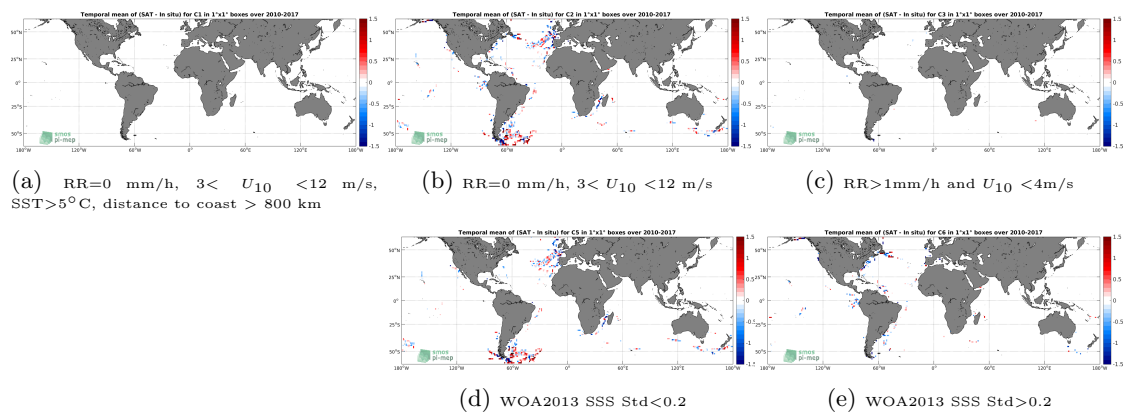
Figure 12: Temporal mean gridded over spatial boxes of size 1^\circ \times 1^\circ of \Delta SSS (SMOS L3 v2 - Daily - 0.5 Deg (CATDS-CECOS-IFREMER) - TSG-GOSUD-Sailing-ship) for 5 different subdatasets corresponding to:RR=0 mm/h, 3 < U_{10} < 12 m/s, SST >5^\circ\text{C} , distance to coast > 800 km (a), RR=0 mm/h, 3 < U_{10} < 12 m/s (b), RR >1 mm/h and U_{10} < 4 m/s (c), WOA2013 SSS Std <0.2 (d), WOA2013 SSS Std >0.2 (e).
