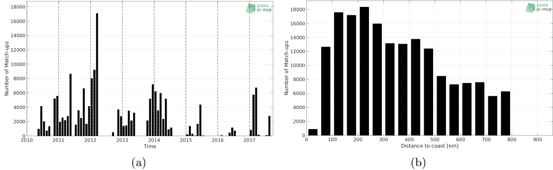
Figure 1: Number of match-ups between TSG-GOSUD-Sailing-ship and SMOS-L3-CATDS-CECOS-IFREMER-V2-1DAY-0.5DEG SSS as a function of time (a) and as function of the distance to coast (b) over the SMOS coastal zone ( \approx 800\text{km} ) 60N-60S Pi-MEP region and for the full satellite product period.
