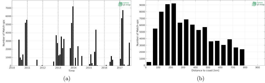
Figure 1: Number of match-ups between TSG-GOSUD-Sailing-ship and SMOS-L3-CATDS-CECOS-IFREMER-V2-1DAY-0.5DEG SSS as a function of time (a) and as function of the distance to coast (b) over the SMOS coastal zone ( \approx 800\text{km} ) 60N-60S Pi-MEP region and for the full satellite product period.
