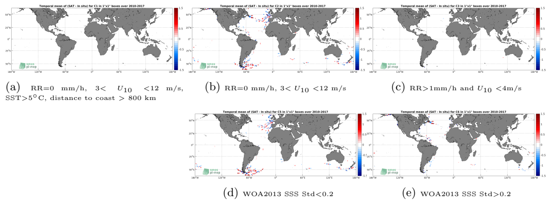
Figure 12: Temporal mean gridded over spatial boxes of size 1^\circ \times 1^\circ of \Delta SSS (SMOS-L3-CATDS-CECOS-IFREMER-V2-1DAY-0.5DEG - TSG-GOSUD-Sailing-ship) for 5 different subdatasets corresponding to:RR=0 mm/h, 3 < U_{10} < 12 m/s, SST >5^\circ C, distance to coast > 800 km (a), RR=0 mm/h, 3 < U_{10} < 12 m/s (b), RR >1 mm/h and U_{10} < 4 m/s (c), WOA2013 SSS Std <0.2 (d), WOA2013 SSS Std >0.2 (e).
