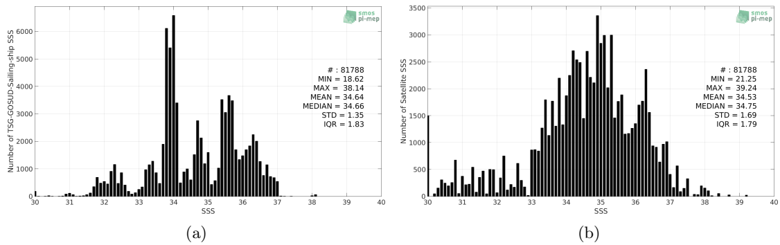
Figure 2: Histograms of SSS from TSG-GOSUD-Sailing-ship (a) and SMOS-L3-CATDS-CECOS-IFREMER-V2-1DAY-0.5DEG (b) considering all match-up pairs per bins of 0.1 over the SMOS coastal zone ( \approx 800\text{km} ) 60N-60S Pi-MEP region and for the full satellite product period.
