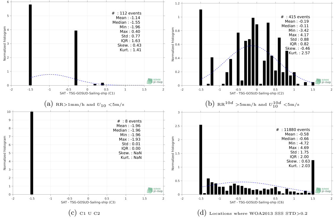
Figure 13: Normalized histogram of \Delta\text{SSS} (SMOS-L3-CATDS-CECOS-IFREMER-V2-1DAY-0.5DEG - TSG-GOSUD-Sailing-ship) for 6 different subdatasets corresponding to: RR > 1mm/h and U_{10} < 5\text{m/s} (a), RR^{10d} > 5\text{mm/h} and U_{10}^{10d} < 5\text{m/s} (b), C1 U C2 (c), Locations where WOA2013 SSS STD > 0.2 (d).
