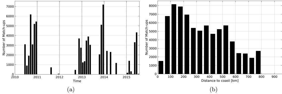
Figure 1: Number of match-ups between TSG-GOSUD-Sailing-ship and SMOS-L3-CATDS-CECOS-IFREMER-V2-1DAY-0.5DEG SSS as a function of time (a) and as function of the distance to coast (b) over the SMOS coastal zone ( \pm 800\text{km} ) 60N-60S Pi-MEP region and for the full satellite product period.
