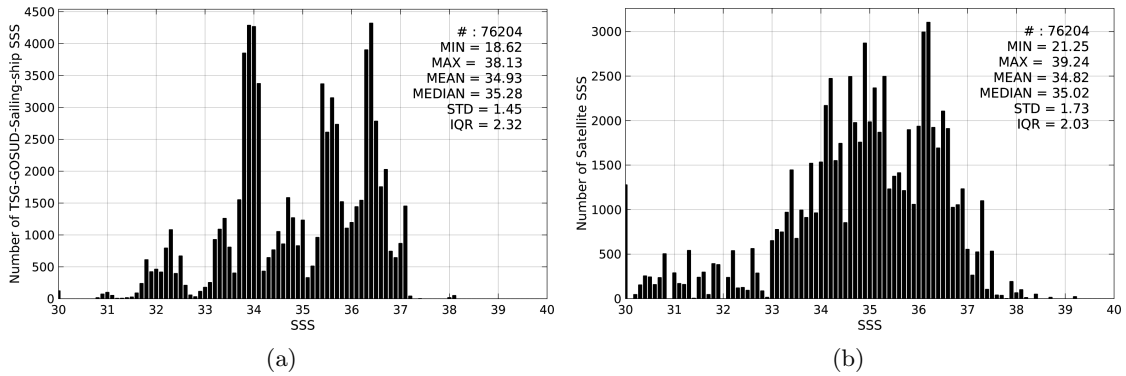
Figure 2: Histograms of SSS from TSG-GOSUD-Sailing-ship (a) and SMOS-L3-CATDS-CECOS-IFREMER-V2-1DAY-0.5DEG (b) considering all match-up pairs per bins of 0.1 over the SMOS coastal zone ( \pm 800\text{km} ) 60N-60S Pi-MEP region and for the full satellite product period.
