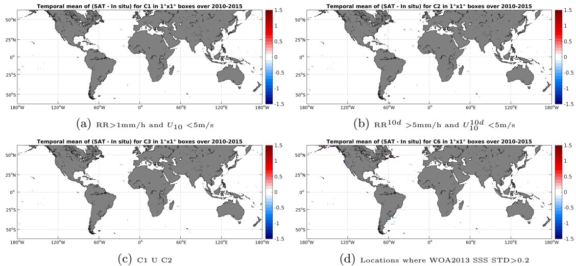
Figure 12: Temporal mean gridded over spatial boxes of size 1^\circ \times 1^\circ of \Delta SSS (SMOS-L3-CATDS-CECOS-IFREMER-V2-1DAY-0.5DEG - TSG-GOSUD-Sailing-ship) for 4 different subdatasets corresponding to: RR > 1\text{mm/h} and U_{10} < 5\text{m/s} (a), RR^{10d} > 5\text{mm/h} and U_{10}^{10d} < 5\text{m/s} (b), C1 U C2 (c), Locations where WOA2013 SSS STD > 0.2 (d).
