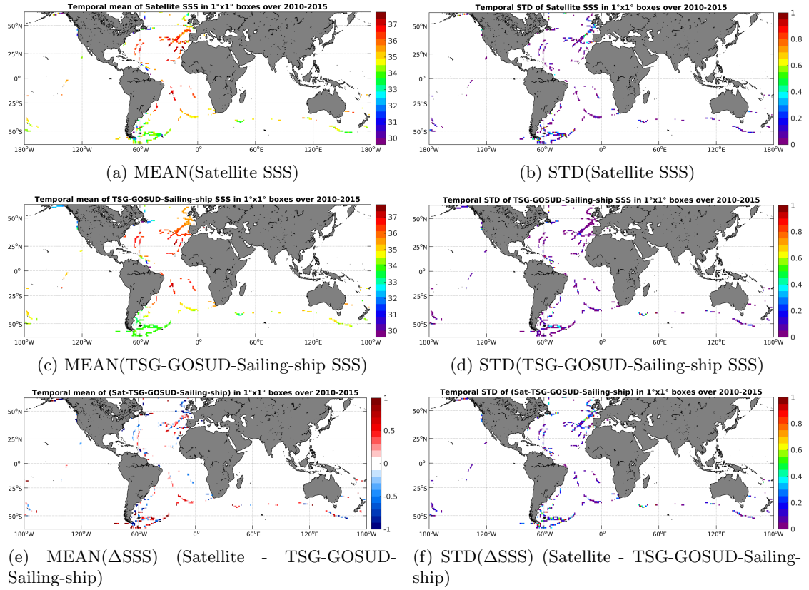
Figure 6: Temporal mean (left) and STD (right) of SSS from SMOS-L3-CATDS-CECOS-IFREMER-V2-1DAY-0.5DEG (top), TSG-GOSUD-Sailing-ship (middle), and of \Delta SSS (Satellite - TSG-GOSUD-Sailing-ship). Only match-up pairs are used to generate these maps.
