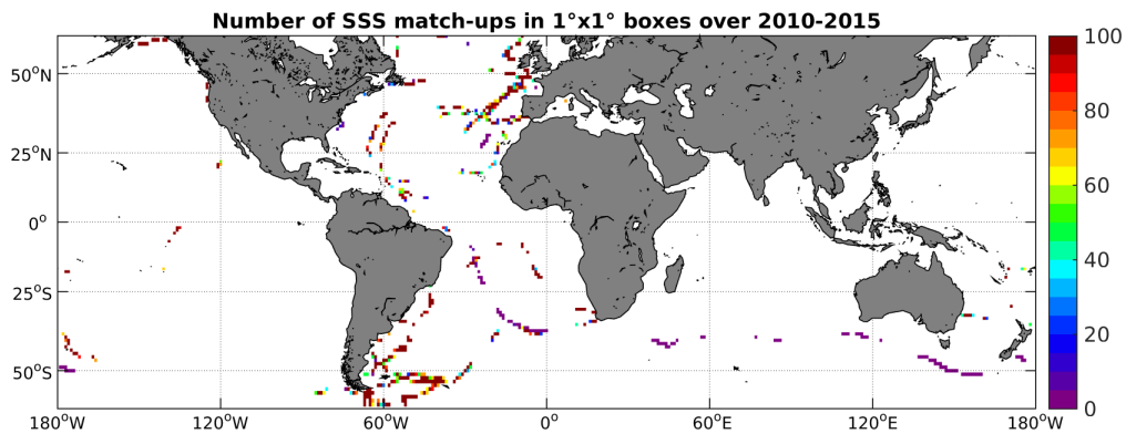
Figure 4: Number of SSS match-ups between TSG-GOSUD-Sailing-ship SSS and the SMOS-L3-CATDS-CECOS-IFREMER-V2-1DAY-0.5DEG SSS product for the SMOS coastal zone ( \pm 800\text{km} ) 60N-60S Pi-MEP region over 1^\circ \times 1^\circ boxes and for the full satellite product period.
