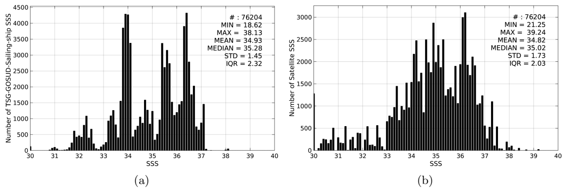
Figure 2: Histograms of SSS from TSG-GOSUD-Sailing-ship (a) and SMOS-L3-CATDS-CECOS-IFREMER-V2-1DAY-0.5deg (b) considering all match-up pairs per bins of 0.1 over the SMOS coastal zone ( \approx 800\text{km} ) 60N-60S Pi-MEP region and for the full satellite product period.
