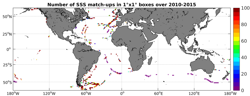
Figure 4: Number of SSS match-ups between TSG-GOSUD-Sailing-ship SSS and the SMOS-L3-CATDS-CECOS-IFREMER-V2-1DAY-0.5deg SSS product for the SMOS coastal zone ( \approx 800\text{km} ) 60N-60S Pi-MEP region over 1^\circ \times 1^\circ boxes and for the full satellite product period.
