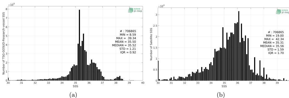
Figure 2: Histograms of SSS from TSG-GOSUD-Research-vessel (a) and SMOS L3 v2 - Daily - 0.5 Deg (CATDS-CECOS-IFREMER) (b) considering all match-up pairs per bins of 0.1 over the SMOS coastal zone (<800km) 60N-60S Pi-MEP region and for the full satellite product period.
