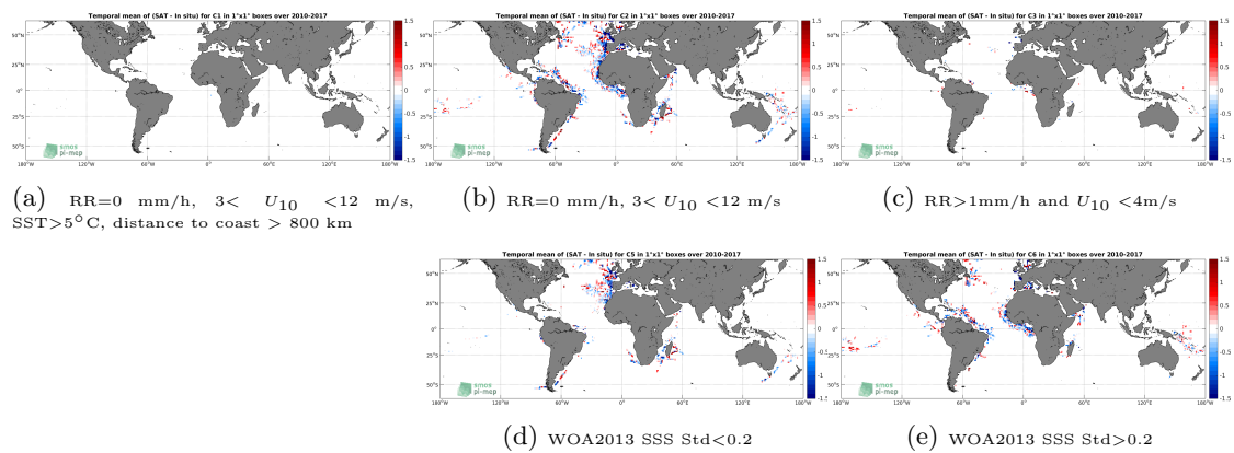
Figure 12: Temporal mean gridded over spatial boxes of size 1^\circ \times 1^\circ of \Delta SSS (SMOS L3 v2 - Daily - 0.5 Deg (CATDS-CECOS-IFREMER) - TSG-GOSUD-Research-vessel) for 5 different subdatasets corresponding to:RR=0 mm/h, 3 < U_{10} < 12 m/s, SST >5^\circ\text{C} , distance to coast > 800 km (a), RR=0 mm/h, 3 < U_{10} < 12 m/s (b), RR >1 mm/h and U_{10} < 4 m/s (c), WOA2013 SSS Std <0.2 (d), WOA2013 SSS Std >0.2 (e).
