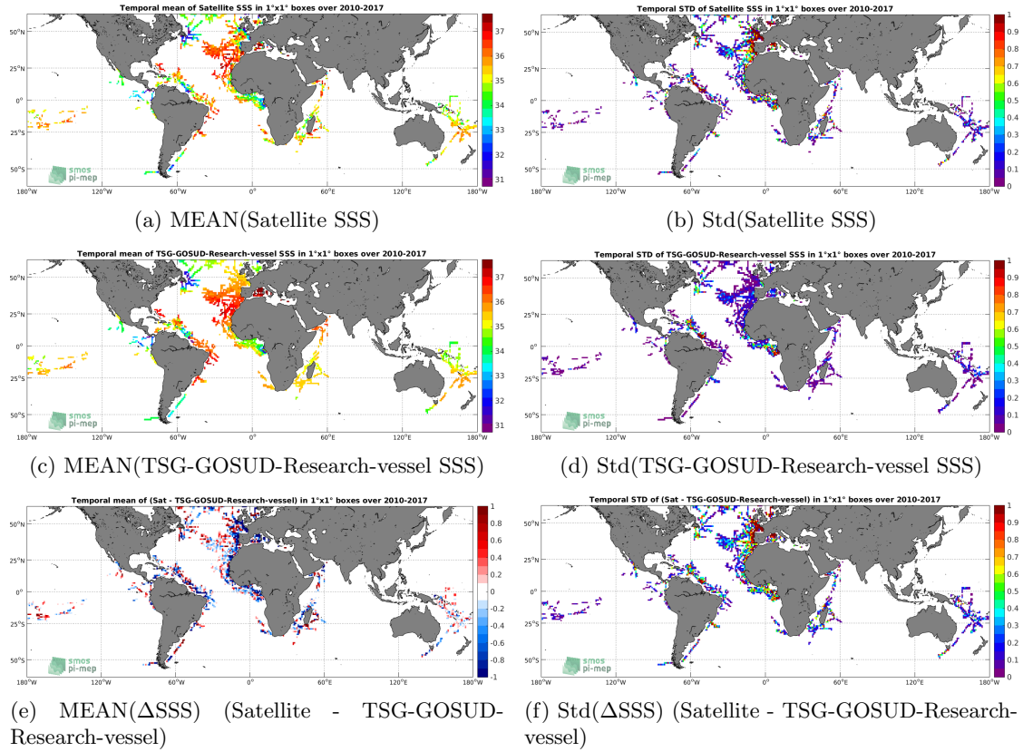
Figure 6: Temporal mean (left) and Std (right) of SSS from SMOS L3 v2 - Daily - 0.5 Deg (CATDS-CECOS-IFREMER) (top), TSG-GOSUD-Research-vessel (middle), and of \Delta SSS (Satellite - TSG-GOSUD-Research-vessel). Only match-up pairs are used to generate these maps.
