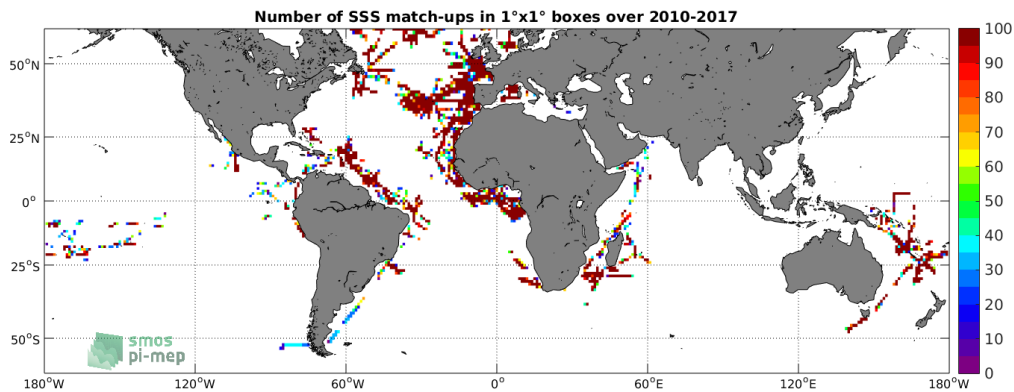
Figure 4: Number of SSS match-ups between TSG-GOSUD-Research-vessel SSS and the SMOS L3 v2 - Daily - 0.5 Deg (CATDS-CECOS-IFREMER) SSS product for the SMOS coastal zone (<800km) 60N-60S Pi-MEP region over 1^\circ \times 1^\circ boxes and for the full satellite product period.
