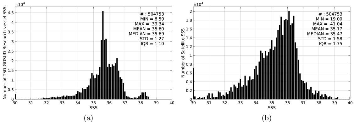
Figure 2: Histograms of SSS from TSG-GOSUD-Research-vessel (a) and SMOS-L3-CATDS-CECOS-IFREMER-V2-1DAY-0.5DEG (b) considering all match-up pairs per bins of 0.1 over the SMOS coastal zone ( \geq 800 km) 60N-60S Pi-MEP region and for the full satellite product period.
