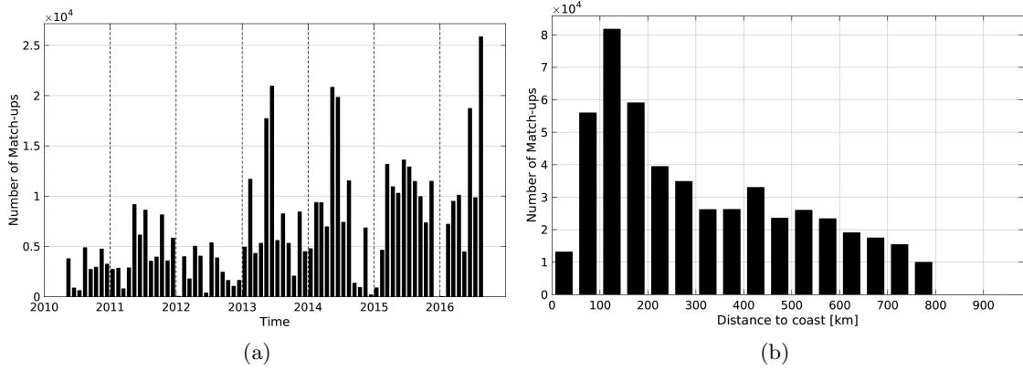
Figure 1: Number of match-ups between TSG-GOSUD-Research-vessel and SMOS-L3-CATDS-CECOS-IFREMER-V2-1DAY-0.5deg SSS as a function of time (a) and as function of the distance to coast (b) over the SMOS coastal zone ( \approx 800 km) 60N-60S Pi-MEP region and for the full satellite product period.
