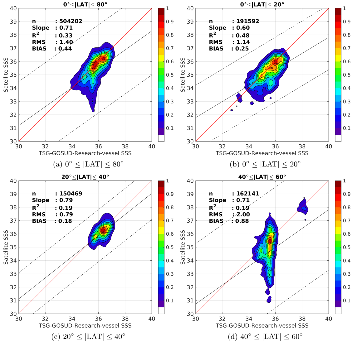
Figure 9: Contour maps of the concentration of SMOS-L3-CATDS-CECOS-IFREMER-V2-1DAY-0.5deg SSS (y-axis) versus TSG-GOSUD-Research-vessel SSS (x-axis) at match-up pairs for different latitude bands. For each plot, the red line shows x=y . The black thin and dashed lines indicate a linear fit through the data cloud and the \pm 95\% confidence levels, respectively. The number match-up pairs n , the slope and R^2 coefficient of the linear fit, the root mean square (RMS) and the mean bias between satellite and in situ data are indicated for each latitude band in each plots.
