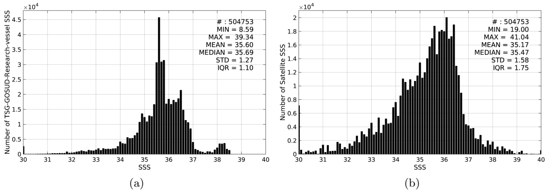
Figure 2: Histograms of SSS from TSG-GOSUD-Research-vessel (a) and SMOS-L3-CATDS-CECOS-IFREMER-V2-1DAY-0.5deg (b) considering all match-up pairs per bins of 0.1 over the SMOS coastal zone ( \approx 800 km) 60N-60S Pi-MEP region and for the full satellite product period.
