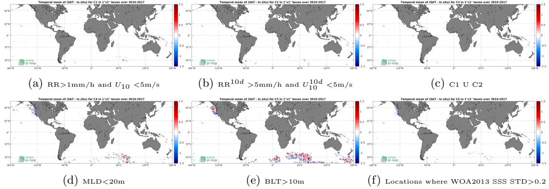
Figure 12: Temporal mean gridded over spatial boxes of size 1^\circ \times 1^\circ of \Delta SSS (SMOS-L3-CATDS-CECOS-IFREMER-V2-1DAY-0.5DEG - Sea mammals) for 6 different subdatasets corresponding to: RR > 1\text{mm/h} and U_{10} < 5\text{m/s} (a), RR^{10d} > 5\text{mm/h} and U_{10}^{10d} < 5\text{m/s} (b), C1 U C2 (c), MLD < 20\text{m} (d), BLT > 10\text{m} (e), Locations where WOA2013 SSS STD > 0.2 (f).
