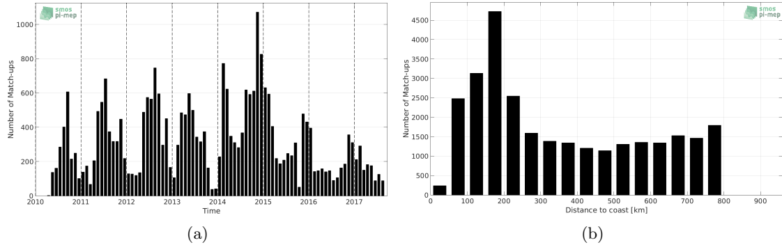
Figure 1: Number of match-ups between Sea mammals and SMOS-L3-CATDS-CECOS-IFREMER-V2-1DAY-0.5DEG SSS as a function of time (a) and as function of the distance to coast (b) over the SMOS coastal zone ( \approx 800 km) 60N-60S Pi-MEP region and for the full satellite product period.
