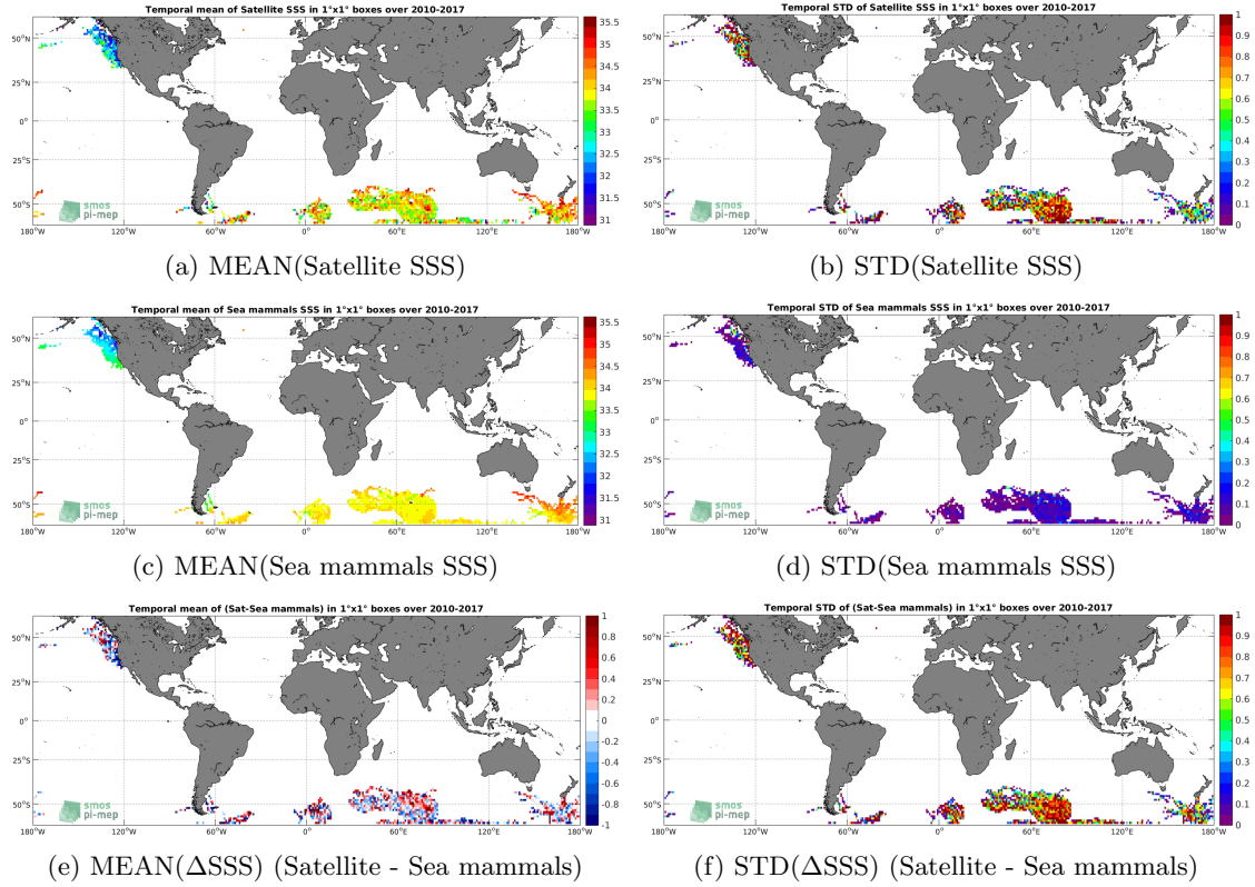
Figure 6: Temporal mean (left) and STD (right) of SSS from SMOS-L3-CATDS-CECOS-IFREMER-V2-1DAY-0.5DEG (top), Sea mammals (middle), and of \Delta SSS (Satellite - Sea mammals). Only match-up pairs are used to generate these maps.
