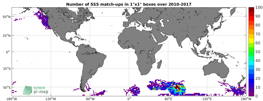
Figure 4: Number of SSS match-ups between Sea mammals SSS and the SMOS-L3-CATDS-CECOS-IFREMER-V2-1DAY-0.5DEG SSS product for the SMOS coastal zone ( \approx 800\text{km} ) 60N-60S Pi-MEP region over 1^\circ \times 1^\circ boxes and for the full satellite product period.
