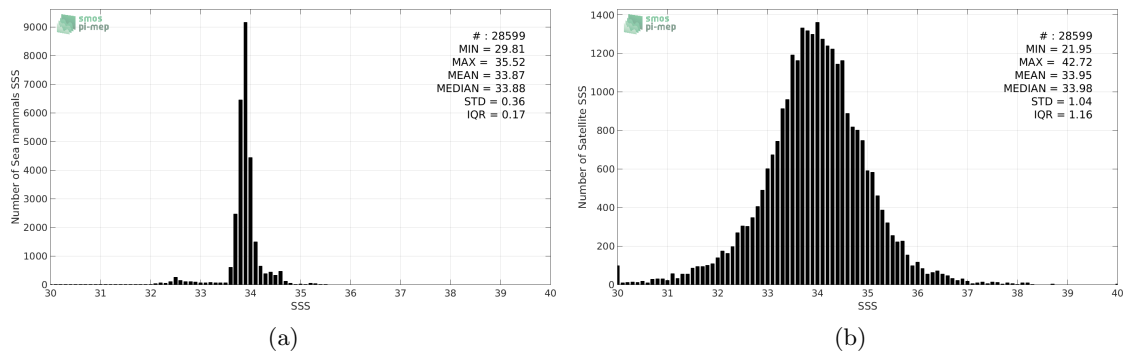
Figure 2: Histograms of SSS from Sea mammals (a) and SMOS-L3-CATDS-CECOS-IFREMER-V2-1DAY-0.5DEG (b) considering all match-up pairs per bins of 0.1 over the SMOS coastal zone ( \approx 800 km) 60N-60S Pi-MEP region and for the full satellite product period.
