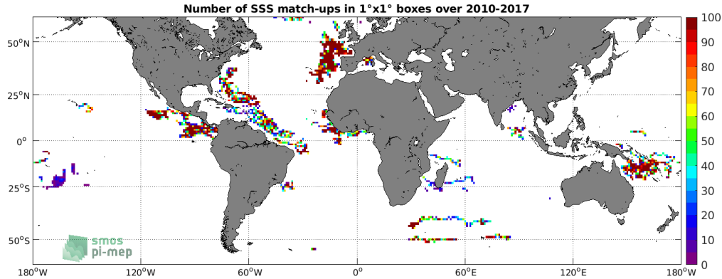
Figure 3: Number of SSS match-ups between Surface drifters SSS and the SMOS SSS L3 v2 - Daily - 0.5 Deg (CATDS-CECOS-IFREMER) SSS product for the SMOS coastal zone ( <800\text{km} ) 60N-60S Pi-MEP region over 1^\circ \times 1^\circ boxes and for the full satellite product period.
