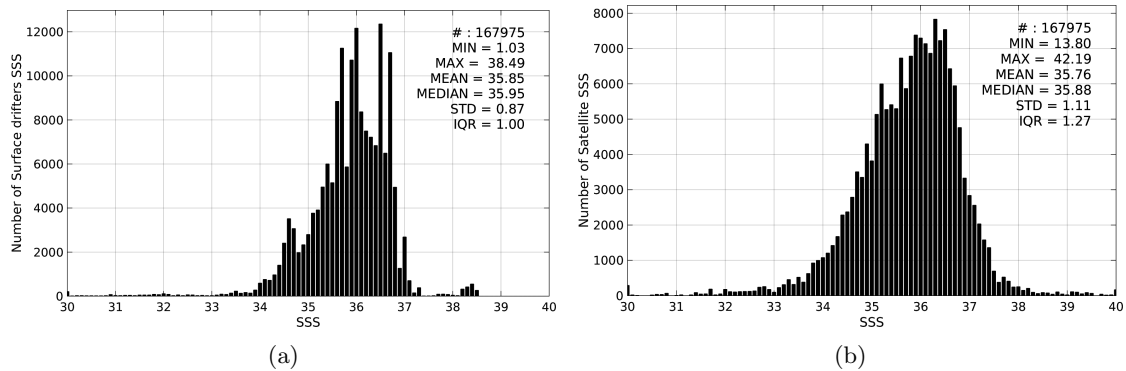
Figure 2: Histograms of SSS from Surface drifters (a) and SMOS-L3-CATDS-CECOS-IFREMER-V2-1DAY-0.5DEG (b) considering all match-up pairs per bins of 0.1 over the SMOS coastal zone ( \geq 800\text{km} ) 60N-60S Pi-MEP region and for the full satellite product period.
