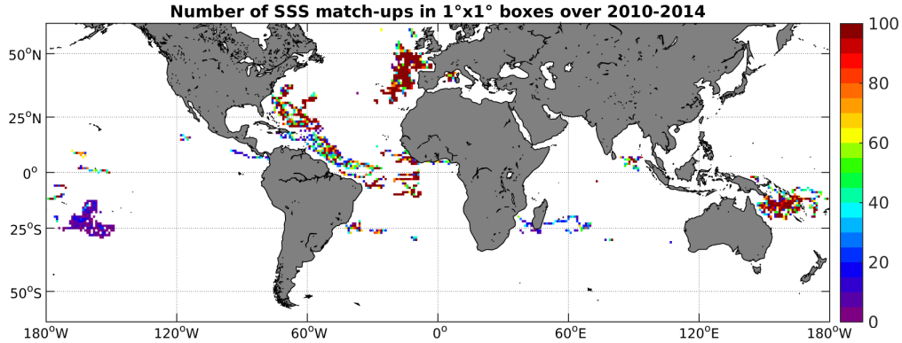
Figure 3: Number of SSS match-ups between Surface drifters SSS and the SMOS-L3-CATDS-CECOS-IFREMER-V2-1DAY-0.5DEG SSS product for the SMOS coastal zone ( \geq 800\text{km} ) 60N-60S Pi-MEP region over 1°x1° boxes and for the full satellite product period.
