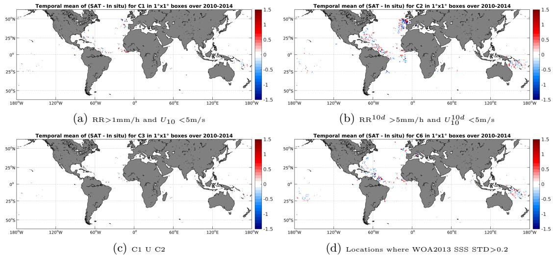
Figure 11: Temporal mean gridded over spatial boxes of size 1^\circ \times 1^\circ of \Delta SSS (SMOS-L3-CATDS-CECOS-IFREMER-V2-1DAY-0.5DEG - Surface drifters) for 4 different subdatasets corresponding to: RR > 1\text{mm/h} and U_{10} < 5\text{m/s} (a), RR^{10d} > 5\text{mm/h} and U_{10}^{10d} < 5\text{m/s} (b), C1 U C2 (c), Locations where WOA2013 SSS STD > 0.2 (d).
