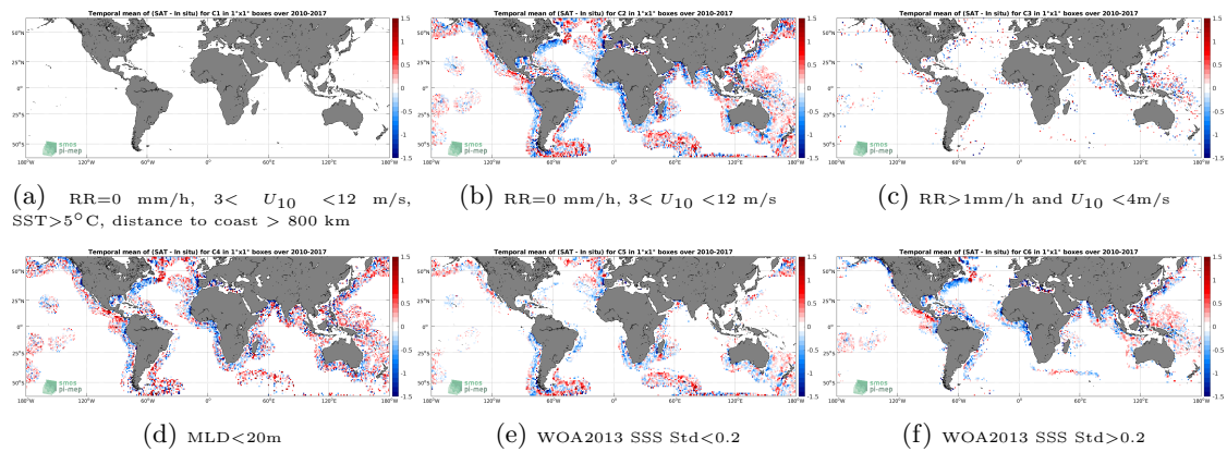
Figure 12: Temporal mean gridded over spatial boxes of size 1^\circ \times 1^\circ of \Delta SSS (SMOS SSS L3 v2 - Daily - 0.5 Deg (CATDS-CECOS-IFREMER) - Argo) for 6 different subdatasets corresponding to: RR=0 mm/h, 3 < U_{10} < 12 m/s, SST > 5^\circ\text{C} , distance to coast > 800 km (a), RR=0 mm/h, 3 < U_{10} < 12 m/s (b), RR > 1 mm/h and U_{10} < 4 m/s (c),MLD < 20 m (d),WOA2013 SSS Std < 0.2 (e),WOA2013 SSS Std > 0.2 (f).
