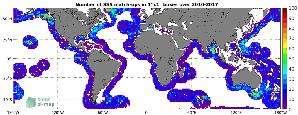
Figure 4: Number of SSS match-ups between Argo SSS and the SMOS SSS L3 v2 - Daily - 0.5 Deg (CATDS-CECOS-IFREMER) SSS product for the SMOS coastal zone (<800km) 60N-60S Pi-MEP region over 1^\circ \times 1^\circ boxes and for the full satellite product period.
