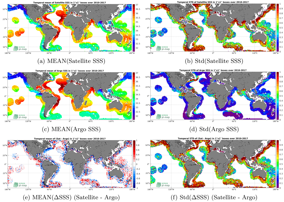
Figure 6: Temporal mean (left) and Std (right) of SSS from SMOS SSS L3 v2 - Daily - 0.5 Deg (CATDS-CECOS-IFREMER) (top), Argo (middle), and of \Delta SSS (Satellite - Argo). Only match-up pairs are used to generate these maps.
