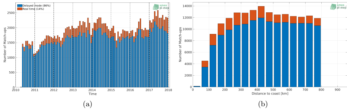
Figure 1: Number of match-ups between Argo and SMOS SSS L3 v2 - Daily - 0.5 Deg (CATDS-CECOS-IFREMER) SSS as a function of time (a) and as function of the distance to coast (b) over the SMOS coastal zone (<800km) 60N-60S Pi-MEP region and for the full satellite product period.
