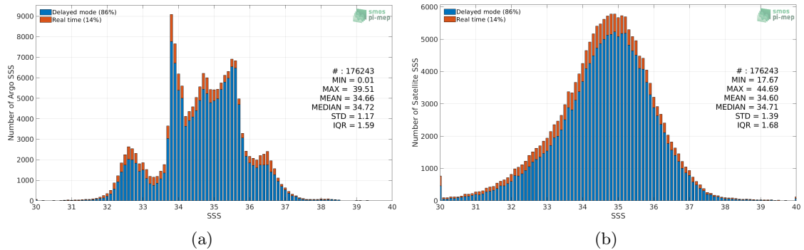
Figure 2: Histograms of SSS from Argo (a) and SMOS SSS L3 v2 - Daily - 0.5 Deg (CATDS-CECOS-IFREMER) (b) considering all match-up pairs per bins of 0.1 over the SMOS coastal zone (<800km) 60N-60S Pi-MEP region and for the full satellite product period.
