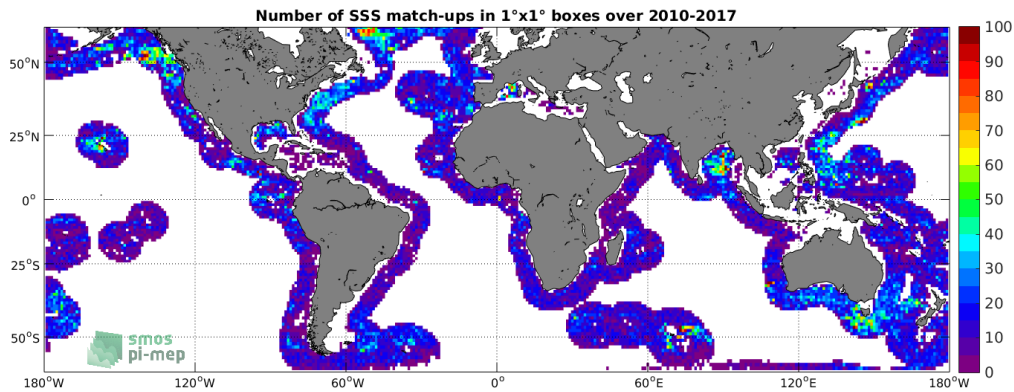
Figure 4: Number of SSS match-ups between Argo SSS and the SMOS-L3-CATDS-CECOS-IFREMER-V2-1DAY-0.5DEG SSS product for the SMOS coastal zone ( \pm 800\text{km} ) 60N-60S Pi-MEP region over 1^\circ \times 1^\circ boxes and for the full satellite product period.
