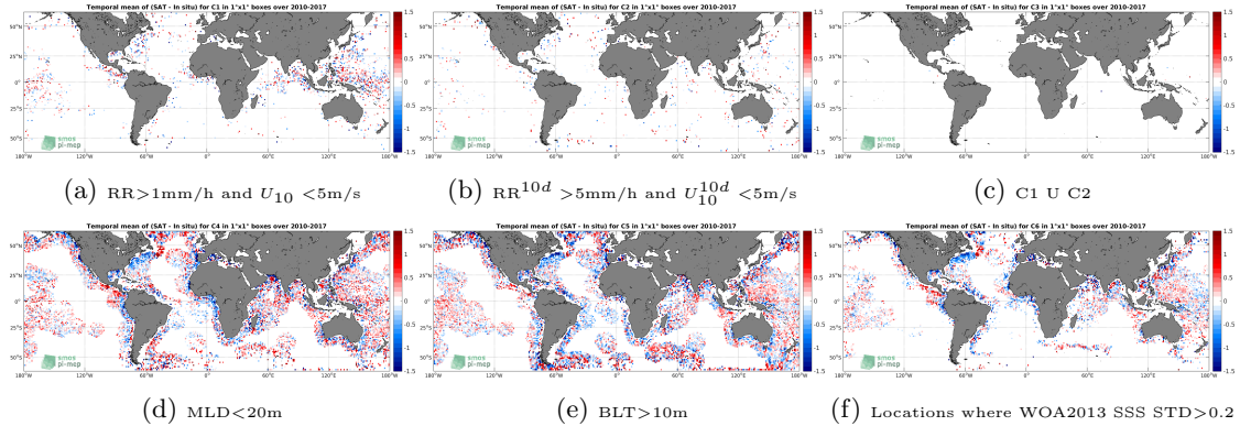
Figure 12: Temporal mean gridded over spatial boxes of size 1^\circ \times 1^\circ of \Delta SSS (SMOS-L3-CATDS-CECOS-IFREMER-V2-1DAY-0.5DEG - Argo) for 6 different subdatasets corresponding to: RR>1mm/h and U_{10} < 5\text{m/s} (a), RR^{10d} > 5\text{mm/h} and U_{10}^{10d} < 5\text{m/s} (b), C1 U C2 (c),MLD<20m (d),BLT>10m (e),Locations where WOA2013 SSS STD>0.2 (f).
