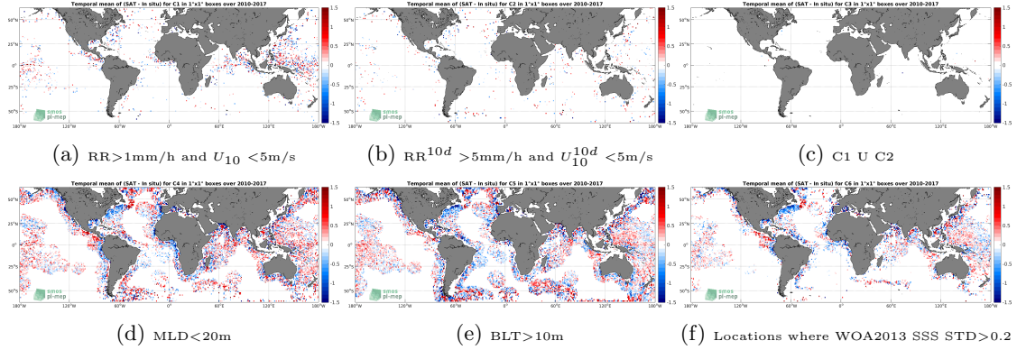
Figure 12: Temporal mean gridded over spatial boxes of size 1°x1° of \Delta SSS (SMOS-L3-CATDS-CECOS-IFREMER-V2-1DAY-0.5DEG - Argo) for 6 different subdatasets corresponding to: RR>1mm/h and U_{10} < 5m/s (a), RR^{10d} > 5mm/h and U_{10}^{10d} < 5m/s (b), C1 U C2 (c),MLD<20m (d),BLT>10m (e),Locations where WOA2013 SSS STD>0.2 (f).
