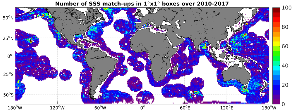
Figure 4: Number of SSS match-ups between Argo SSS and the SMOS-L3-CATDS-CECOS-IFREMER-V2-1DAY-0.5deg SSS product for the SMOS coastal zone ( \geq 800\text{km} ) 60N-60S Pi-MEP region over 1^\circ \times 1^\circ boxes and for the full satellite product period.
