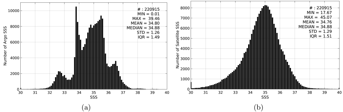
Figure 2: Histograms of SSS from Argo (a) and SMOS-L3-CATDS-CECOS-IFREMER-V2-1DAY-0.5deg (b) considering all match-up pairs per bins of 0.1 over the SMOS coastal zone ( \approx 800\text{km} ) 60N-60S Pi-MEP region and for the full satellite product period.
