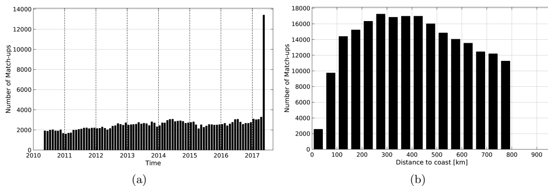
Figure 1: Number of match-ups between Argo and SMOS-L3-CATDS-CECOS-IFREMER-V2-1DAY-0.5deg SSS as a function of time (a) and as function of the distance to coast (b) over the SMOS coastal zone ( \pm 800 km) 60N-60S Pi-MEP region and for the full satellite product period.
