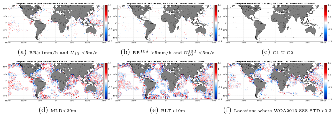
Figure 12: Temporal mean gridded over spatial boxes of size 1^\circ \times 1^\circ of \Delta SSS (SMOS-L3-CATDS-CECOS-IFREMER-V2-1DAY-0.5deg - Argo) for 6 different subdatasets corresponding to: RR > 1\text{mm/h} and U_{10} < 5\text{m/s} (a), RR^{10d} > 5\text{mm/h} and U_{10}^{10d} < 5\text{m/s} (b), C1 U C2 (c), MLD < 20\text{m} (d), BLT > 10\text{m} (e), Locations where WOA2013 SSS STD > 0.2 (f).
