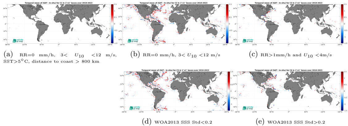
Figure 12: Temporal mean gridded over spatial boxes of size 1^\circ \times 1^\circ of \Delta SSS (SMOS SSS L3 v335 - Monthly - 25 km (CATDS-CPDC) - TSG (SAMOS)) for 5 different subdatasets corresponding to:RR=0 mm/h, 3 < U_{10} < 12 m/s, SST >5^\circ C, distance to coast > 800 km (a), RR=0 mm/h, 3 < U_{10} < 12 m/s (b), RR >1 mm/h and U_{10} < 4 m/s (c), WOA2013 SSS Std <0.2 (d), WOA2013 SSS Std >0.2 (e).
