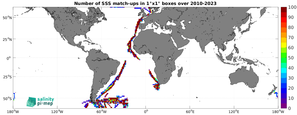
Figure 5: Number of SSS match-ups between TSG (Polarstern) SSS and the SMOS SSS L3 v335 - Monthly - 25 km (CATDS-CPDC) SSS product for the SMOS coastal zone (<800km) 60N-60S Pi-MEP region over 1^\circ \times 1^\circ boxes and for the full satellite product period.
