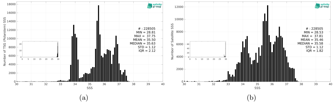
Figure 3: Histograms of SSS from TSG (Polarstern) (a) and SMOS SSS L3 v335 - Monthly - 25 km (CATDS-CPDC) (b) considering all match-up pairs per bins of 0.1 over the SMOS coastal zone (<800km) 60N-60S Pi-MEP region and for the full satellite product period.
