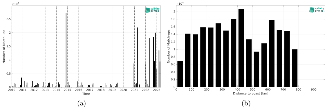
Figure 2: Number of match-ups between TSG (Polarstern) and SMOS SSS L3 v335 - Monthly - 25 km (CATDS-CPDC) SSS as a function of time (a) and as function of the distance to coast (b) over the SMOS coastal zone (<800km) 60N-60S Pi-MEP region and for the full satellite product period.
