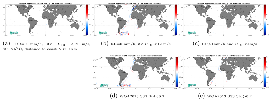
Figure 14: Temporal mean gridded over spatial boxes of size 1^\circ \times 1^\circ of \Delta\text{SSS} (SMOS SSS L3 v335 - Monthly - 25 km (CATDS-CPDC) - TSG (Polarstern)) for 5 different subdatasets corresponding to:RR=0 mm/h, 3 < U_{10} < 12 m/s, SST>5°C, distance to coast > 800 km (a), RR=0 mm/h, 3 < U_{10} < 12 m/s (b), RR>1mm/h and U_{10} < 4 m/s (c), WOA2013 SSS Std<0.2 (d), WOA2013 SSS Std>0.2 (e).
