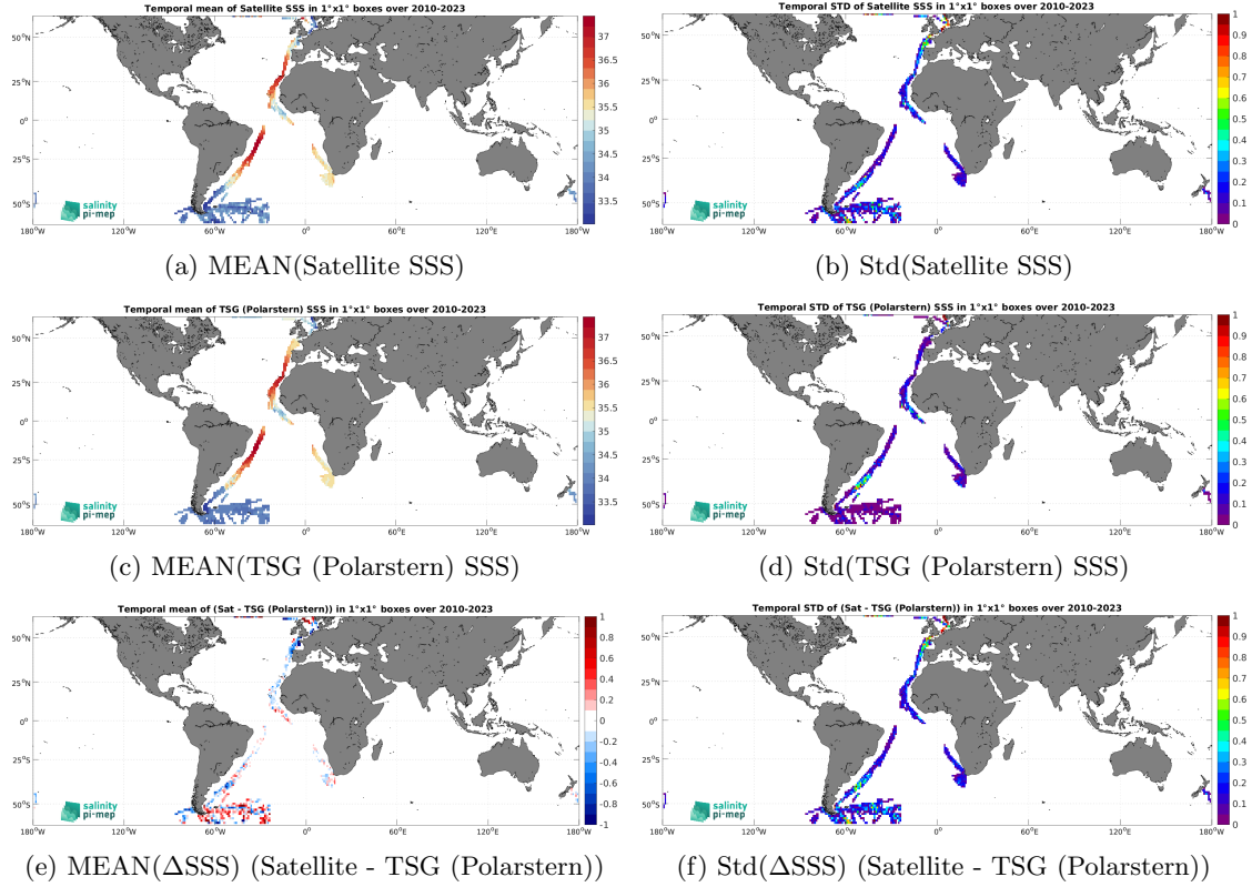
Figure 7: Temporal mean (left) and Std (right) of SSS from SMOS SSS L3 v335 - Monthly - 25 km (CATDS-CPDC) (top), TSG (Polarstern) (middle), and of \Delta SSS (Satellite - TSG (Polarstern)). Only match-up pairs are used to generate these maps.
