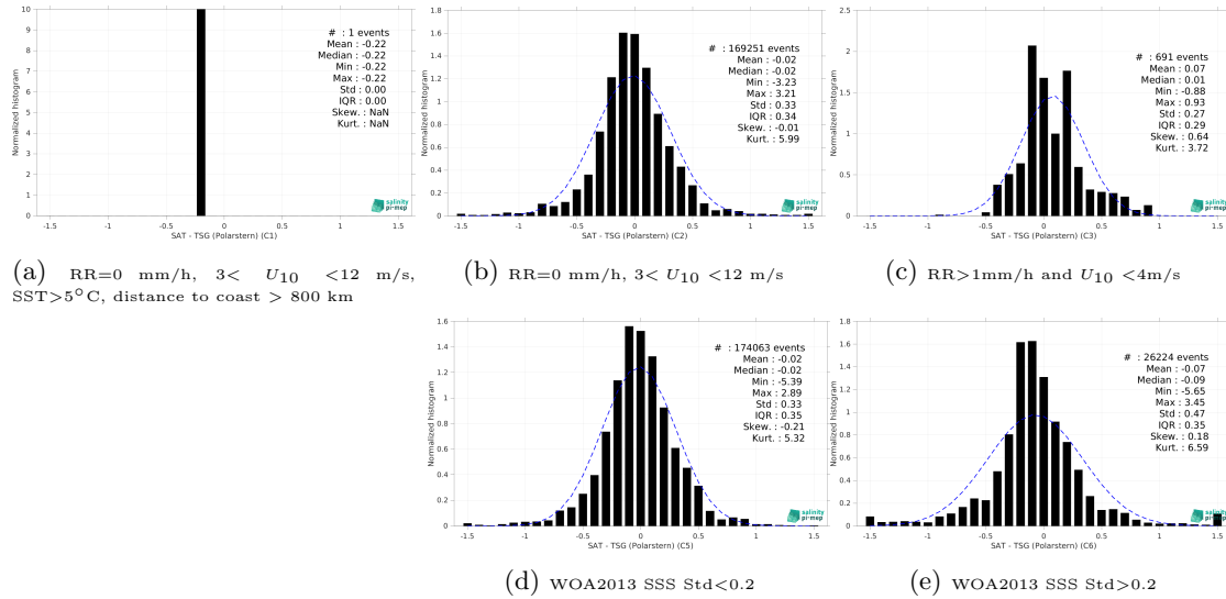
Figure 15: Normalized histogram of \Delta\text{SSS} (SMOS SSS L3 v335 - Monthly - 25 km (CATDS-CPDC) - TSG (Polarstern)) for 5 different subdatasets corresponding to: RR=0 mm/h, 3 < U_{10} < 12 m/s, SST>5°C, distance to coast > 800 km (a), RR=0 mm/h, 3 < U_{10} < 12 m/s (b), RR>1mm/h and U_{10} < 4 m/s (c), WOA2013 SSS Std<0.2 (d), WOA2013 SSS Std>0.2 (e).
