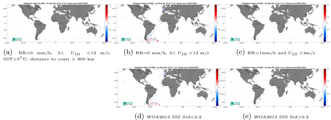
Figure 12: Temporal mean gridded over spatial boxes of size 1^\circ \times 1^\circ of \Delta\text{SSS} (SMOS SSS L3 v335 - Monthly - 25 km (CATDS-CPDC) - TSG (Polarstern)) for 5 different subdatasets corresponding to:RR=0 mm/h, 3 < U_{10} < 12 m/s, SST >5^\circ\text{C} , distance to coast > 800 km (a), RR=0 mm/h, 3 < U_{10} < 12 m/s (b), RR >1 mm/h and U_{10} < 4 m/s (c), WOA2013 SSS Std <0.2 (d), WOA2013 SSS Std >0.2 (e).
