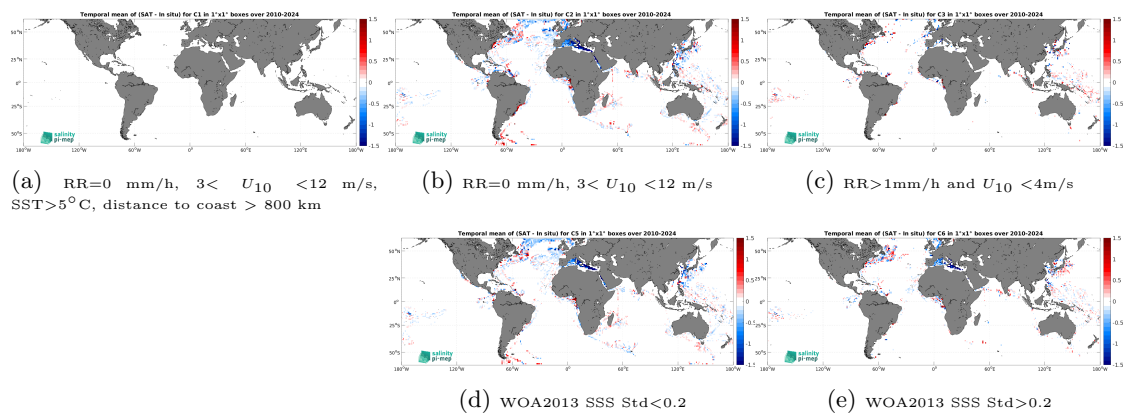
Figure 14: Temporal mean gridded over spatial boxes of size 1^\circ \times 1^\circ of \Delta SSS (SMOS SSS L3 v335 - Monthly - 25 km (CATDS-CPDC) - TSG (LEGOS-DM)) for 5 different subdatasets corresponding to: RR=0 mm/h, 3 < U_{10} < 12 m/s, SST > 5^\circ\text{C} , distance to coast > 800 km (a), RR=0 mm/h, 3 < U_{10} < 12 m/s (b), RR > 1 mm/h and U_{10} < 4 m/s (c), WOA2013 SSS Std < 0.2 (d), WOA2013 SSS Std > 0.2 (e).
