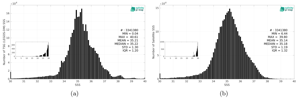
Figure 3: Histograms of SSS from TSG (LEGOS-DM) (a) and SMOS SSS L3 v335 - Monthly - 25 km (CATDS-CPDC) (b) considering all match-up pairs per bins of 0.1 over the SMOS coastal zone (<800km) 60N-60S Pi-MEP region and for the full satellite product period.
