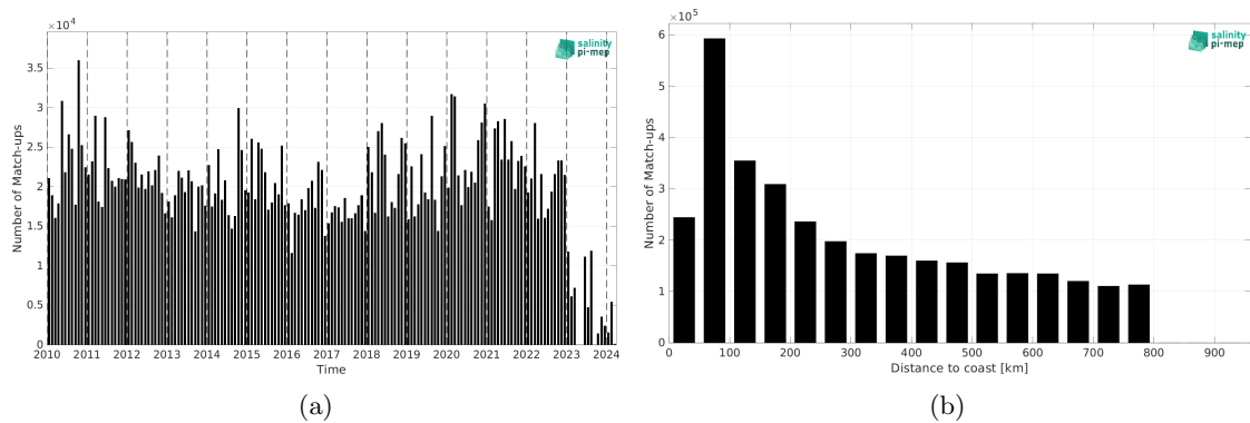
Figure 2: Number of match-ups between TSG (LEGOS-DM) and SMOS SSS L3 v335 - Monthly - 25 km (CATDS-CPDC) SSS as a function of time (a) and as function of the distance to coast (b) over the SMOS coastal zone (<800km) 60N-60S Pi-MEP region and for the full satellite product period.
