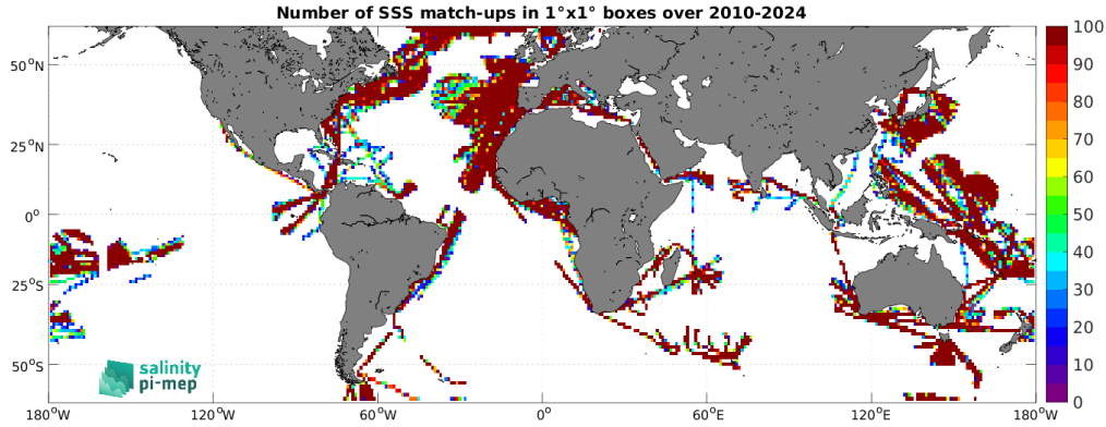
Figure 5: Number of SSS match-ups between TSG (LEGOS-DM) SSS and the SMOS SSS L3 v335 - Monthly - 25 km (CATDS-CPDC) SSS product for the SMOS coastal zone (<800km) 60N-60S Pi-MEP region over 1^\circ \times 1^\circ boxes and for the full satellite product period.
