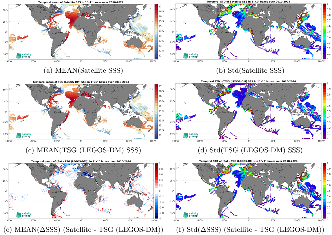
Figure 7: Temporal mean (left) and Std (right) of SSS from SMOS SSS L3 v335 - Monthly - 25 km (CATDS-CPDC) (top), TSG (LEGOS-DM) (middle), and of \Delta SSS (Satellite - TSG (LEGOS-DM)). Only match-up pairs are used to generate these maps.
