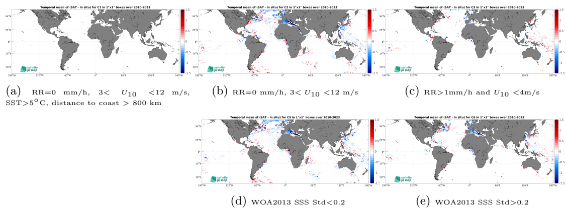
Figure 14: Temporal mean gridded over spatial boxes of size 1^\circ \times 1^\circ of \Delta\text{SSS} (SMOS SSS L3 v335 - Monthly - 25 km (CATDS-CPDC) - TSG (LEGOS-DM)) for 5 different subdatasets corresponding to: RR=0 mm/h, 3 < U_{10} < 12 m/s, SST > 5°C, distance to coast > 800 km (a), RR=0 mm/h, 3 < U_{10} < 12 m/s (b), RR > 1mm/h and U_{10} < 4 m/s (c), WOA2013 SSS Std < 0.2 (d), WOA2013 SSS Std > 0.2 (e).
