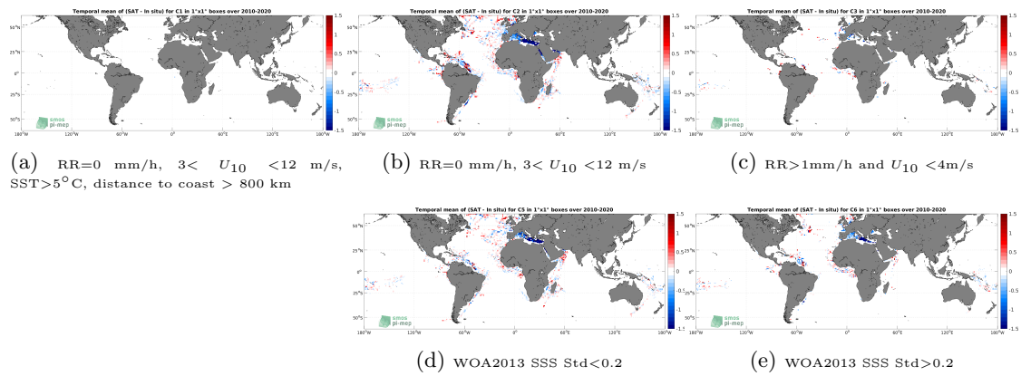
Figure 12: Temporal mean gridded over spatial boxes of size 1^\circ \times 1^\circ of \Delta SSS (SMOS SSS L3 v335 - Monthly - 25 km (CATDS-CPDC) - TSG (GOSUD-Research-vessel)) for 5 different subdatasets corresponding to:RR=0 mm/h, 3 < U_{10} < 12 m/s, SST >5^\circ C, distance to coast > 800 km (a), RR=0 mm/h, 3 < U_{10} < 12 m/s (b), RR >1 mm/h and U_{10} < 4 m/s (c), WOA2013 SSS Std <0.2 (d), WOA2013 SSS Std >0.2 (e).
