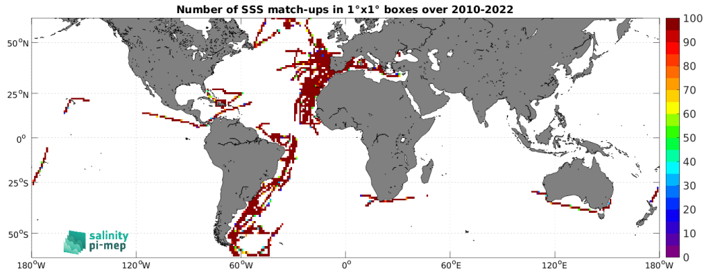
Figure 5: Number of SSS match-ups between TSG (CSIC-UTM) SSS and the SMOS SSS L3 v335 - Monthly - 25 km (CATDS-CPDC) SSS product for the SMOS coastal zone (<800km) 60N-60S Pi-MEP region over 1^\circ \times 1^\circ boxes and for the full satellite product period.
