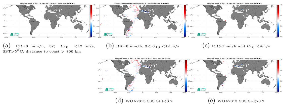
Figure 14: Temporal mean gridded over spatial boxes of size 1^\circ \times 1^\circ of \Delta SSS (SMOS SSS L3 v335 - Monthly - 25 km (CATDS-CPDC) - TSG (CSIC-UTM)) for 5 different subdatasets corresponding to:RR=0 mm/h, 3 < U_{10} < 12 m/s, SST >5^\circ C, distance to coast > 800 km (a), RR=0 mm/h, 3 < U_{10} < 12 m/s (b), RR >1 mm/h and U_{10} < 4 m/s (c), WOA2013 SSS Std <0.2 (d), WOA2013 SSS Std >0.2 (e).
