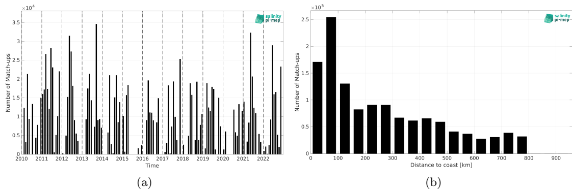
Figure 2: Number of match-ups between TSG (CSIC-UTM) and SMOS SSS L3 v335 - Monthly - 25 km (CATDS-CPDC) SSS as a function of time (a) and as function of the distance to coast (b) over the SMOS coastal zone (<800km) 60N-60S Pi-MEP region and for the full satellite product period.
