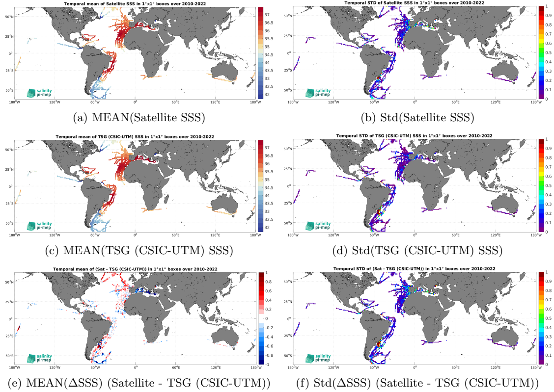
Figure 7: Temporal mean (left) and Std (right) of SSS from SMOS SSS L3 v335 - Monthly - 25 km (CATDS-CPDC) (top), TSG (CSIC-UTM) (middle), and of \Delta SSS (Satellite - TSG (CSIC-UTM)). Only match-up pairs are used to generate these maps.
