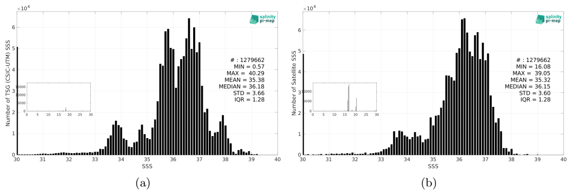
Figure 3: Histograms of SSS from TSG (CSIC-UTM) (a) and SMOS SSS L3 v335 - Monthly - 25 km (CATDS-CPDC) (b) considering all match-up pairs per bins of 0.1 over the SMOS coastal zone (<800km) 60N-60S Pi-MEP region and for the full satellite product period.
