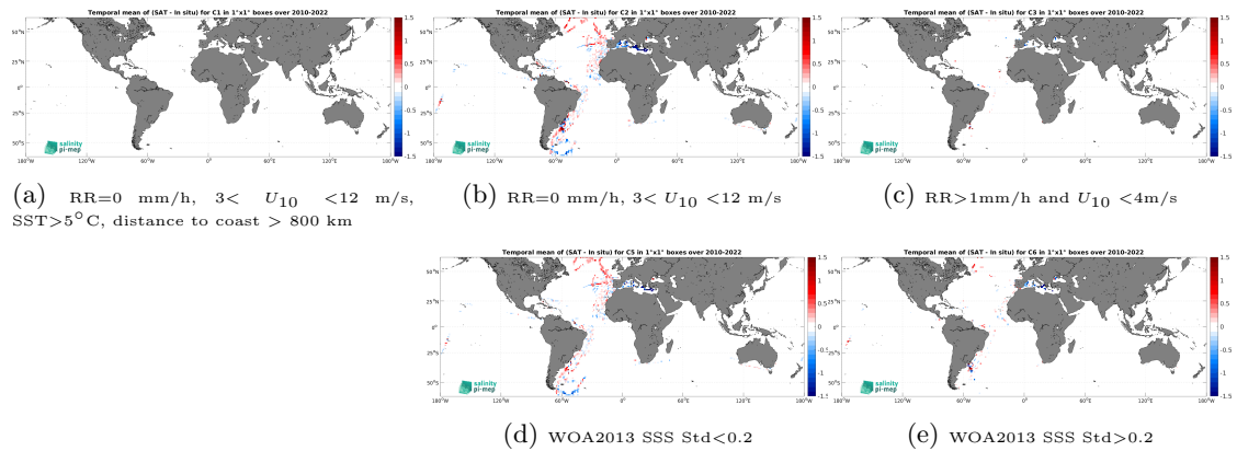
Figure 12: Temporal mean gridded over spatial boxes of size 1^\circ \times 1^\circ of \Delta\text{SSS} (SMOS SSS L3 v335 - Monthly - 25 km (CATDS-CPDC) - TSG (CSIC-UTM)) for 5 different subdatasets corresponding to:RR=0 mm/h, 3 < U_{10} < 12 m/s, SST >5^\circ\text{C} , distance to coast > 800 km (a), RR=0 mm/h, 3 < U_{10} < 12 m/s (b), RR >1 mm/h and U_{10} < 4 m/s (c), WOA2013 SSS Std <0.2 (d), WOA2013 SSS Std >0.2 (e).
