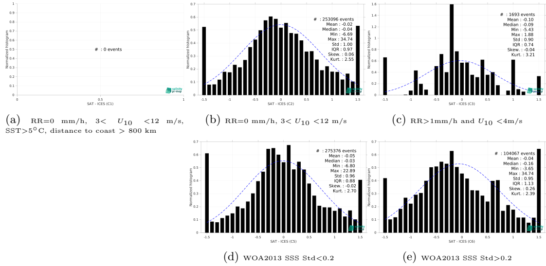
Figure 15: Normalized histogram of \Delta SSS (SMOS SSS L3 v335 - Monthly - 25 km (CATDS-CPDC) - ICES) for 5 different subdatasets corresponding to: RR=0 mm/h, 3 < U_{10} < 12 m/s, SST > 5°C, distance to coast > 800 km (a), RR=0 mm/h, 3 < U_{10} < 12 m/s (b), RR > 1mm/h and U_{10} < 4 m/s (c), WOA2013 SSS Std < 0.2 (d), WOA2013 SSS Std > 0.2 (e).
