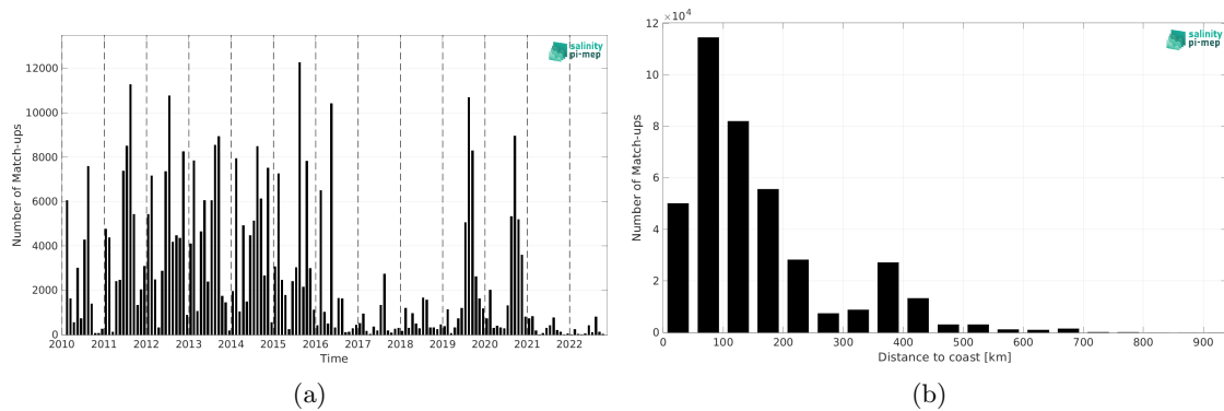
Figure 2: Number of match-ups between ICES and SMOS SSS L3 v335 - Monthly - 25 km (CATDS-CPDC) SSS as a function of time (a) and as function of the distance to coast (b) over the SMOS coastal zone (<800km) 60N-60S Pi-MEP region and for the full satellite product period.
