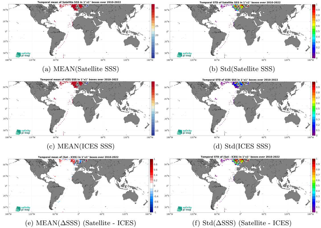
Figure 7: Temporal mean (left) and Std (right) of SSS from SMOS SSS L3 v335 - Monthly - 25 km (CATDS-CPDC) (top), ICES (middle), and of \Delta SSS (Satellite - ICES). Only match-up pairs are used to generate these maps.
