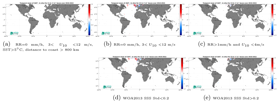
Figure 14: Temporal mean gridded over spatial boxes of size 1^\circ \times 1^\circ of \Delta SSS (SMOS SSS L3 v335 - Monthly - 25 km (CATDS-CPDC) - ICES) for 5 different subdatasets corresponding to:RR=0 mm/h, 3 < U_{10} < 12 m/s, SST >5^\circ\text{C} , distance to coast > 800 km (a), RR=0 mm/h, 3 < U_{10} < 12 m/s (b), RR >1 mm/h and U_{10} < 4 m/s (c), WOA2013 SSS Std <0.2 (d), WOA2013 SSS Std >0.2 (e).
