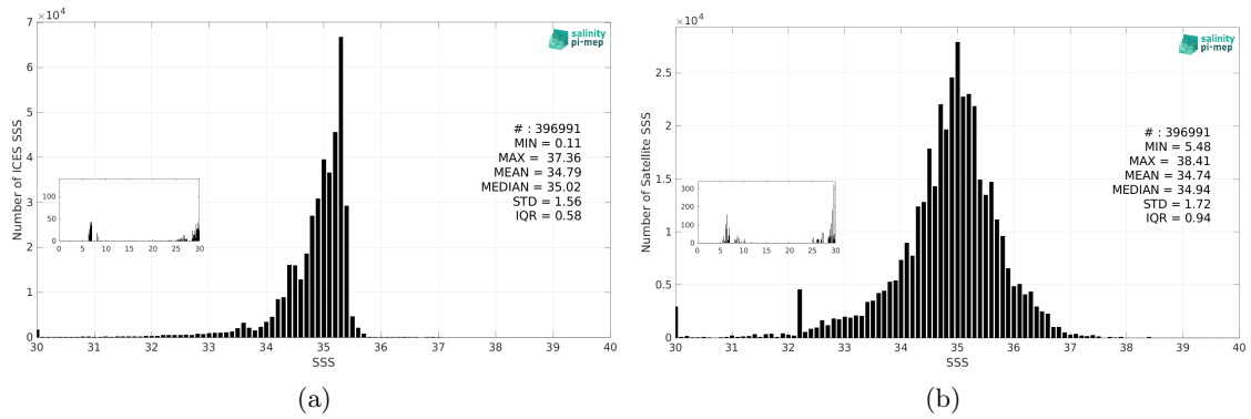
Figure 3: Histograms of SSS from ICES (a) and SMOS SSS L3 v335 - Monthly - 25 km (CATDS-CPDC) (b) considering all match-up pairs per bins of 0.1 over the SMOS coastal zone (<800km) 60N-60S Pi-MEP region and for the full satellite product period.
