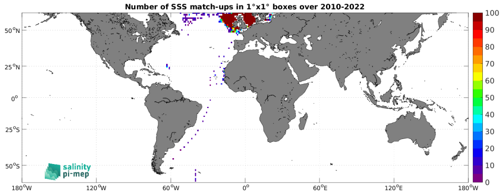
Figure 4: Number of SSS match-ups between ICES SSS and the SMOS SSS L3 v335 - Monthly - 25 km (CATDS-CPDC) SSS product for the SMOS coastal zone (<800km) 60N-60S Pi-MEP region over 1^{\circ} \times 1^{\circ} boxes and for the full satellite product period.
