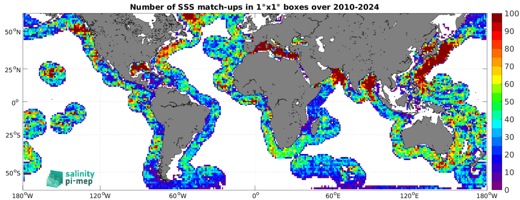
Figure 5: Number of SSS match-ups between Argo SSS and the SMOS SSS L3 v335 - Monthly - 25 km (CATDS-CPDC) SSS product for the SMOS coastal zone (<800km) 60N-60S Pi-MEP region over 1^\circ \times 1^\circ boxes and for the full satellite product period.
