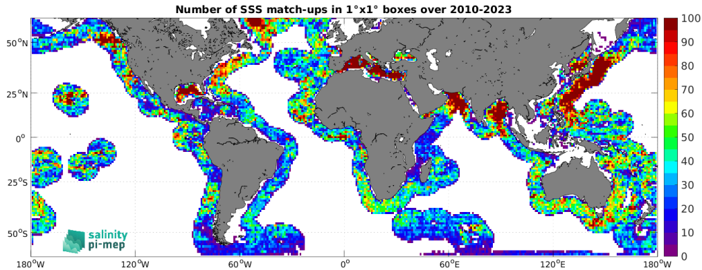
Figure 4: Number of SSS match-ups between Argo SSS and the SMOS SSS L3 v335 - Monthly - 25 km (CATDS-CPDC) SSS product for the SMOS coastal zone (<800km) 60N-60S Pi-MEP region over 1^{\circ} \times 1^{\circ} boxes and for the full satellite product period.
