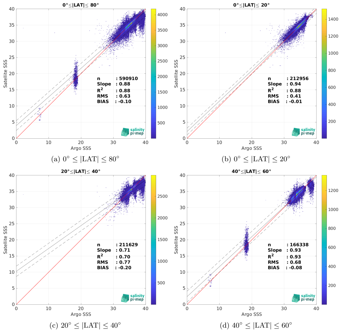
Figure 9: Contour maps of the concentration of SMOS SSS L3 v335 - Monthly - 25 km (CATDS-CPDC) SSS (y-axis) versus Argo SSS (x-axis) at match-up pairs for different latitude bands. For each plot, the red line shows x=y . The black thin and dashed lines indicate a linear fit through the data cloud and the \pm 95\% confidence levels, respectively. The number match-up pairs n , the slope and R^2 coefficient of the linear fit, the root mean square (RMS) and the mean bias between satellite and in situ data are indicated for each latitude band in each plots.
