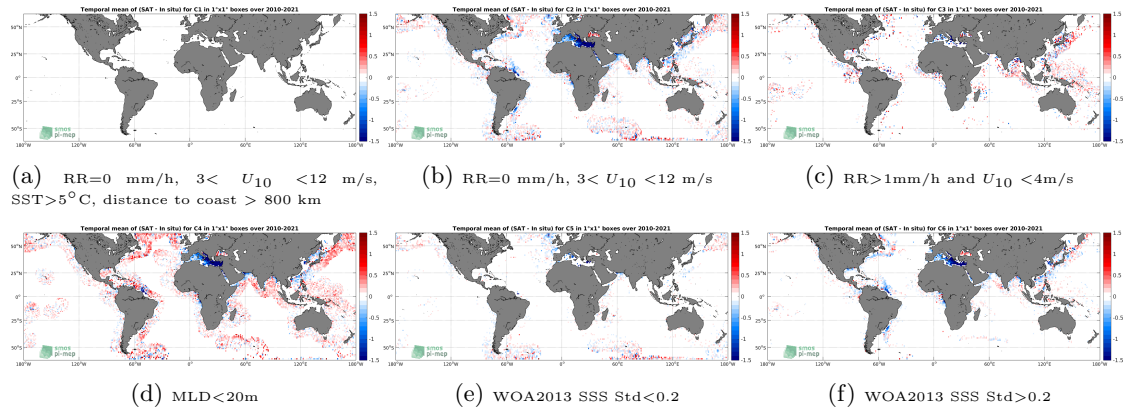
Figure 12: Temporal mean gridded over spatial boxes of size 1^\circ \times 1^\circ of \Delta SSS (SMOS SSS L3 v335 - Monthly - 25 km (CATDS-CPDC) - Argo) for 6 different subdatasets corresponding to: RR=0 mm/h, 3 < U_{10} < 12 m/s, SST > 5°C, distance to coast > 800 km (a), RR=0 mm/h, 3 < U_{10} < 12 m/s (b), RR > 1mm/h and U_{10} < 4 m/s (c), MLD < 20m (d), WOA2013 SSS Std < 0.2 (e), WOA2013 SSS Std > 0.2 (f).
