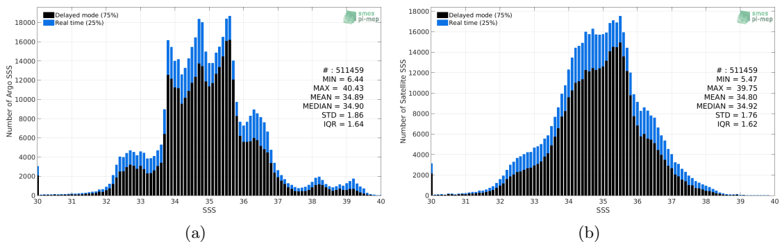
Figure 2: Histograms of SSS from Argo (a) and SMOS SSS L3 v335 - Monthly - 25 km (CATDS-CPDC) (b) considering all match-up pairs per bins of 0.1 over the SMOS coastal zone (<800km) 60N-60S Pi-MEP region and for the full satellite product period.
