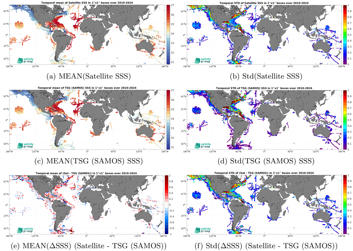
Figure 7: Temporal mean (left) and Std (right) of SSS from SMOS SSS L3 v335 - 10 Days - 25 km (CATDS-CPDC) (top), TSG (SAMOS) (middle), and of \Delta SSS (Satellite - TSG (SAMOS)). Only match-up pairs are used to generate these maps.
