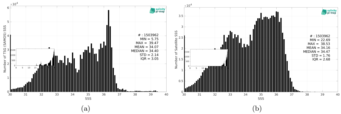
Figure 3: Histograms of SSS from TSG (SAMOS) (a) and SMOS SSS L3 v335 - 10 Days - 25 km (CATDS-CPDC) (b) considering all match-up pairs per bins of 0.1 over the SMOS coastal zone (<800km) 60N-60S Pi-MEP region and for the full satellite product period.
