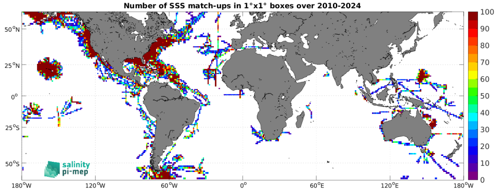
Figure 5: Number of SSS match-ups between TSG (SAMOS) SSS and the SMOS SSS L3 v335 - 10 Days - 25 km (CATDS-CPDC) SSS product for the SMOS coastal zone (<800km) 60N-60S Pi-MEP region over 1^\circ \times 1^\circ boxes and for the full satellite product period.
