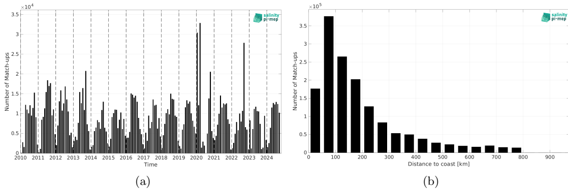
Figure 2: Number of match-ups between TSG (SAMOS) and SMOS SSS L3 v335 - 10 Days - 25 km (CATDS-CPDC) SSS as a function of time (a) and as function of the distance to coast (b) over the SMOS coastal zone (<800km) 60N-60S Pi-MEP region and for the full satellite product period.
