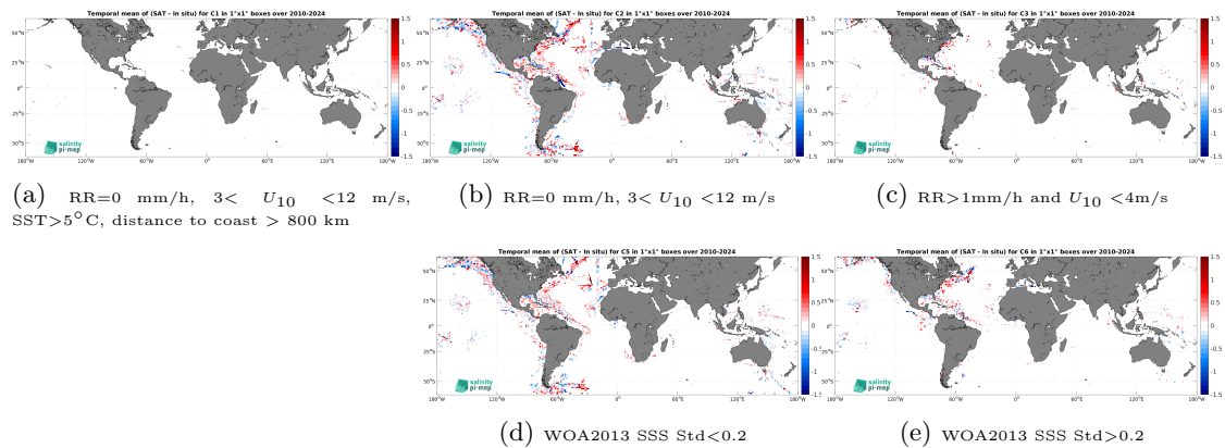
Figure 14: Temporal mean gridded over spatial boxes of size 1^\circ \times 1^\circ of \Delta\text{SSS} (SMOS SSS L3 v335 - 10 Days - 25 km (CATDS-CPDC) - TSG (SAMOS)) for 5 different subdatasets corresponding to:RR=0 mm/h, 3 < U_{10} < 12 m/s, SST >5^\circ\text{C} , distance to coast > 800 km (a), RR=0 mm/h, 3 < U_{10} < 12 m/s (b), RR >1 mm/h and U_{10} < 4 m/s (c), WOA2013 SSS Std <0.2 (d), WOA2013 SSS Std >0.2 (e).
