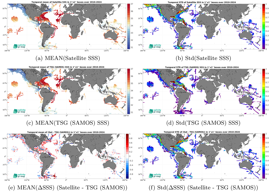
Figure 7: Temporal mean (left) and Std (right) of SSS from SMOS SSS L3 v335 - 10 Days - 25 km (CATDS-CPDC) (top), TSG (SAMOS) ( in situ ) dataset (middle), and of \Delta SSS (Satellite - TSG (SAMOS)). Only match-up pairs are used to generate these maps.
