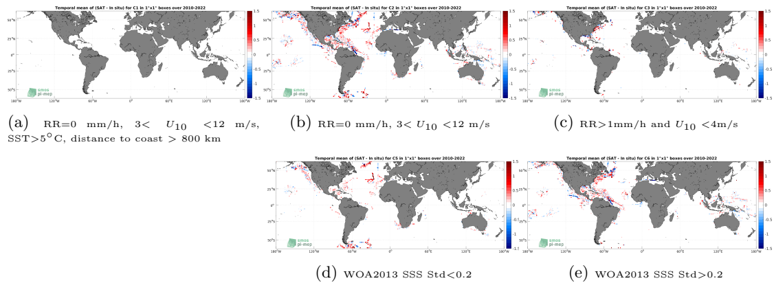
Figure 12: Temporal mean gridded over spatial boxes of size 1^\circ \times 1^\circ of \Delta SSS (SMOS SSS L3 v335 - 10 Days - 25 km (CATDS-CPDC) - TSG (SAMOS)) for 5 different subdatasets corresponding to:RR=0 mm/h, 3 < U_{10} < 12 m/s, SST >5^\circ C, distance to coast > 800 km (a), RR=0 mm/h, 3 < U_{10} < 12 m/s (b), RR >1 mm/h and U_{10} < 4 m/s (c), WOA2013 SSS Std <0.2 (d), WOA2013 SSS Std >0.2 (e).
