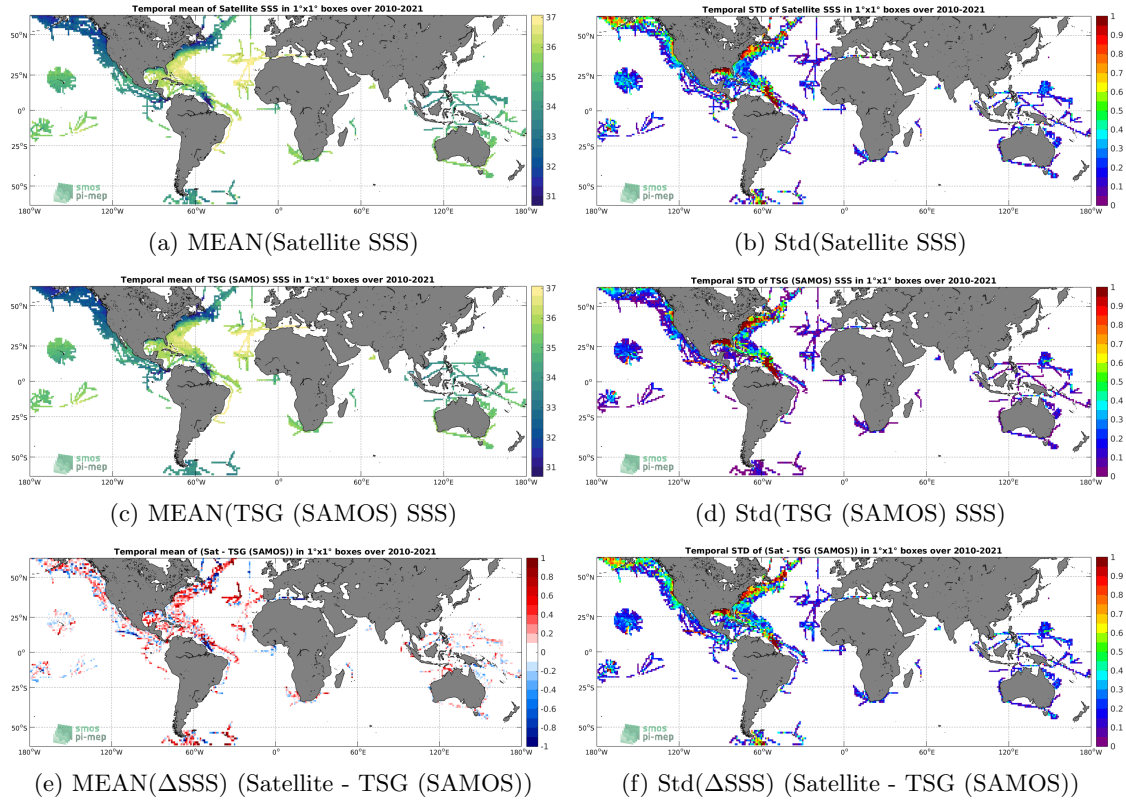
Figure 6: Temporal mean (left) and Std (right) of SSS from SMOS SSS L3 v335 - 10 Days - 25 km (CATDS-CPDC) (top), TSG (SAMOS) (middle), and of \Delta SSS (Satellite - TSG (SAMOS)). Only match-up pairs are used to generate these maps.
