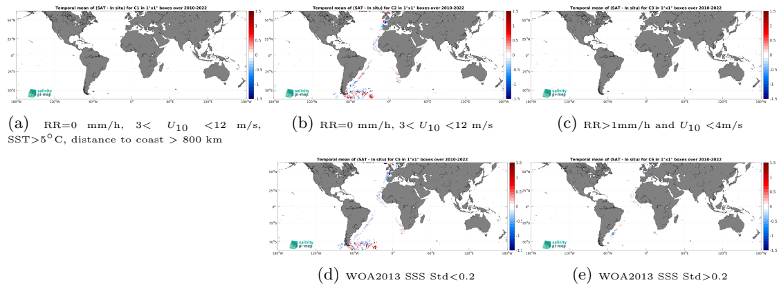
Figure 12: Temporal mean gridded over spatial boxes of size 1^\circ \times 1^\circ of \Delta\text{SSS} (SMOS SSS L3 v335 - 10 Days - 25 km (CATDS-CPDC) - TSG (Polarstern)) for 5 different subdatasets corresponding to:RR=0 mm/h, 3 < U_{10} < 12 m/s, SST >5^\circ\text{C} , distance to coast > 800 km (a), RR=0 mm/h, 3 < U_{10} < 12 m/s (b), RR >1 mm/h and U_{10} < 4 m/s (c), WOA2013 SSS Std <0.2 (d), WOA2013 SSS Std >0.2 (e).
