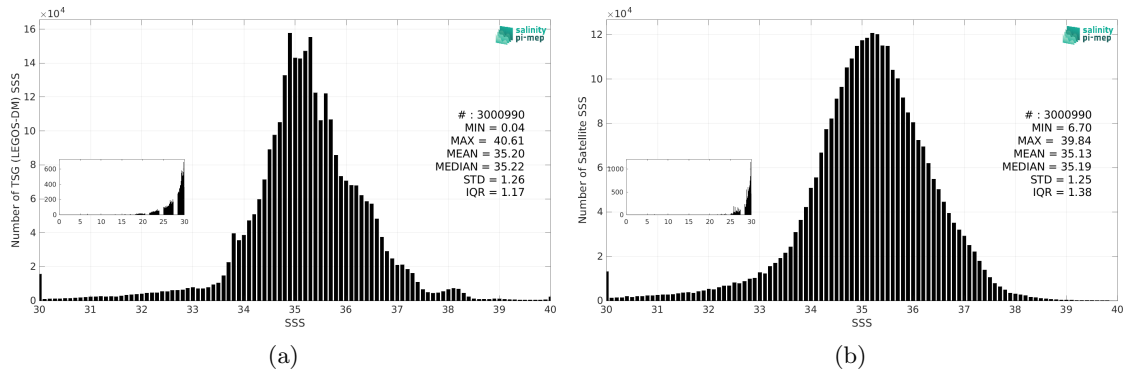
Figure 3: Histograms of SSS from TSG (LEGOS-DM) (a) and SMOS SSS L3 v335 - 10 Days - 25 km (CATDS-CPDC) (b) considering all match-up pairs per bins of 0.1 over the SMOS coastal zone (<800km) 60N-60S Pi-MEP region and for the full satellite product period.
