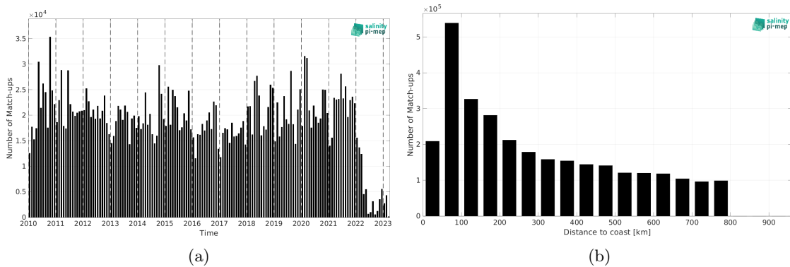
Figure 2: Number of match-ups between TSG (LEGOS-DM) and SMOS SSS L3 v335 - 10 Days - 25 km (CATDS-CPDC) SSS as a function of time (a) and as function of the distance to coast (b) over the SMOS coastal zone (<800km) 60N-60S Pi-MEP region and for the full satellite product period.
