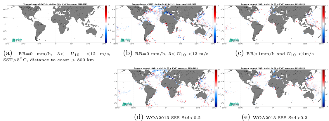
Figure 14: Temporal mean gridded over spatial boxes of size 1^\circ \times 1^\circ of \Delta SSS (SMOS SSS L3 v335 - 10 Days - 25 km (CATDS-CPDC) - TSG (LEGOS-DM)) for 5 different subdatasets corresponding to:RR=0 mm/h, 3 < U_{10} < 12 m/s, SST >5^\circ C, distance to coast > 800 km (a), RR=0 mm/h, 3 < U_{10} < 12 m/s (b), RR >1 mm/h and U_{10} < 4 m/s (c), WOA2013 SSS Std <0.2 (d), WOA2013 SSS Std >0.2 (e).
