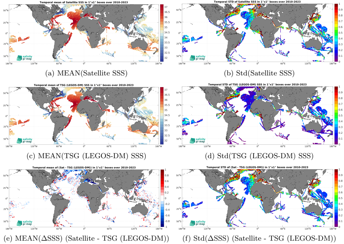
Figure 7: Temporal mean (left) and Std (right) of SSS from SMOS SSS L3 v335 - 10 Days - 25 km (CATDS-CPDC) (top), TSG (LEGOS-DM) (middle), and of \Delta SSS (Satellite - TSG (LEGOS-DM)). Only match-up pairs are used to generate these maps.
