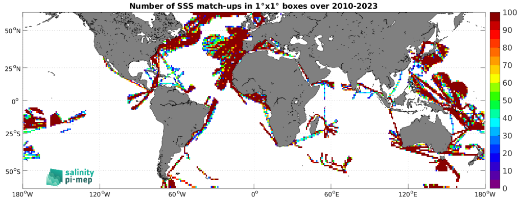
Figure 5: Number of SSS match-ups between TSG (LEGOS-DM) SSS and the SMOS SSS L3 v335 - 10 Days - 25 km (CATDS-CPDC) SSS product for the SMOS coastal zone (<800km) 60N-60S Pi-MEP region over 1^{\circ} \times 1^{\circ} boxes and for the full satellite product period.
