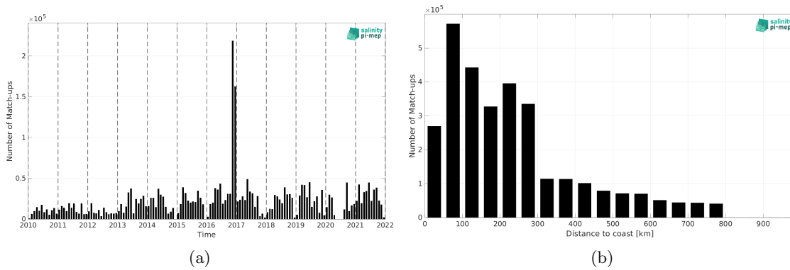
Figure 1: Number of match-ups between TSG (GOSUD-Research-vessel) and SMOS SSS L3 v335 - 10 Days - 25 km (CATDS-CPDC) SSS as a function of time (a) and as function of the distance to coast (b) over the SMOS coastal zone (<800km) 60N-60S Pi-MEP region and for the full satellite product period.
