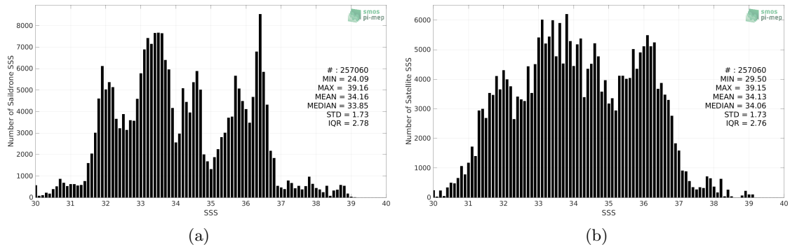
Figure 2: Histograms of SSS from Saildrone (a) and SMOS SSS L3 v335 - 10 Days - 25 km (CATDS-CPDC) (b) considering all match-up pairs per bins of 0.1 over the SMOS coastal zone (<800km) 60N-60S Pi-MEP region and for the full satellite product period.
