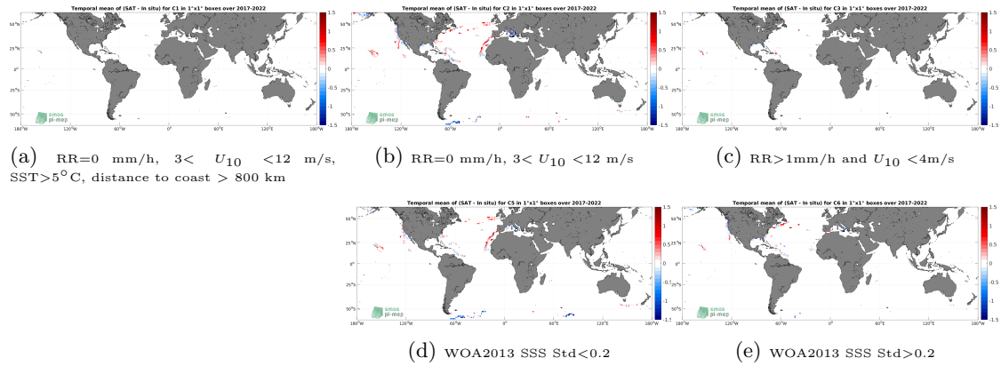
Figure 12: Temporal mean gridded over spatial boxes of size 1^\circ \times 1^\circ of \Delta SSS (SMOS SSS L3 v335 - 10 Days - 25 km (CATDS-CPDC) - Saildrone) for 5 different subdatasets corresponding to:RR=0 mm/h, 3 < U_{10} < 12 m/s, SST >5^\circ C, distance to coast > 800 km (a), RR=0 mm/h, 3 < U_{10} < 12 m/s (b), RR >1 mm/h and U_{10} < 4 m/s (c), WOA2013 SSS Std <0.2 (d), WOA2013 SSS Std >0.2 (e).
