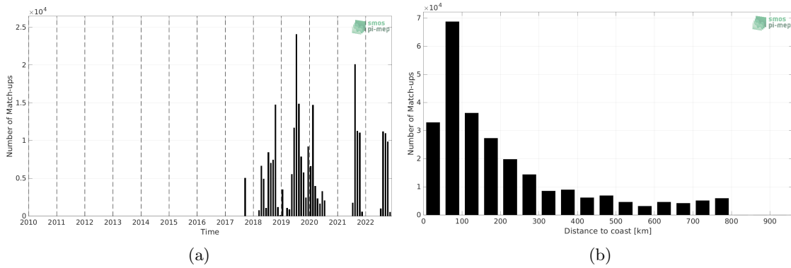
Figure 1: Number of match-ups between Saildrone and SMOS SSS L3 v335 - 10 Days - 25 km (CATDS-CPDC) SSS as a function of time (a) and as function of the distance to coast (b) over the SMOS coastal zone (<800km) 60N-60S Pi-MEP region and for the full satellite product period.
