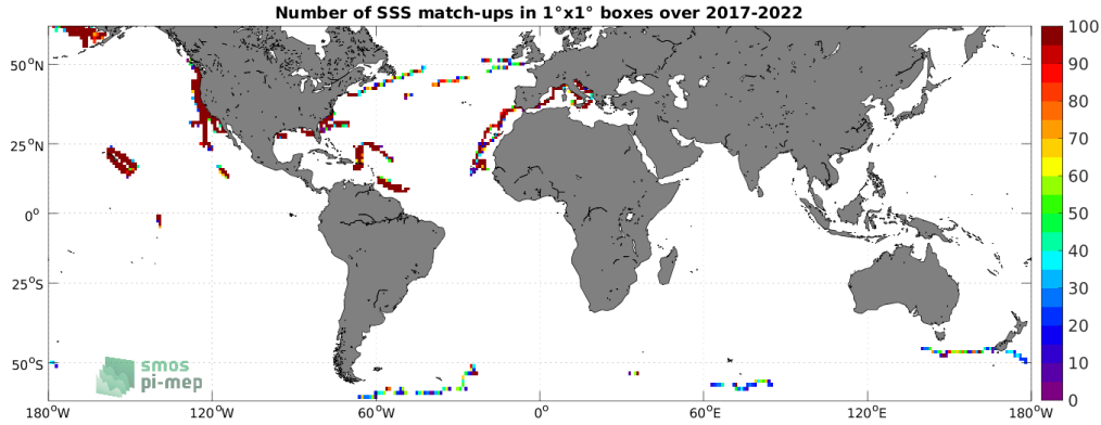
Figure 4: Number of SSS match-ups between Saildrone SSS and the SMOS SSS L3 v335 - 10 Days - 25 km (CATDS-CPDC) SSS product for the SMOS coastal zone (<800km) 60N-60S Pi-MEP region over 1^{\circ} \times 1^{\circ} boxes and for the full satellite product period.
