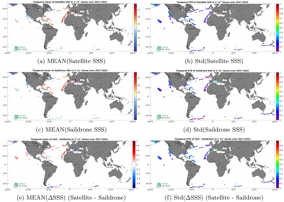
Figure 6: Temporal mean (left) and Std (right) of SSS from SMOS SSS L3 v335 - 10 Days - 25 km (CATDS-CPDC) (top), Saildrone (middle), and of \Delta SSS (Satellite - Saildrone). Only match-up pairs are used to generate these maps.
