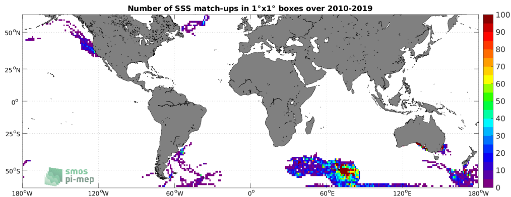
Figure 4: Number of SSS match-ups between Marine mammals SSS and the SMOS SSS L3 v335 - 10 Days - 25 km (CATDS-CPDC) SSS product for the SMOS coastal zone (<800km) 60N-60S Pi-MEP region over 1°×1° boxes and for the full satellite product period.
