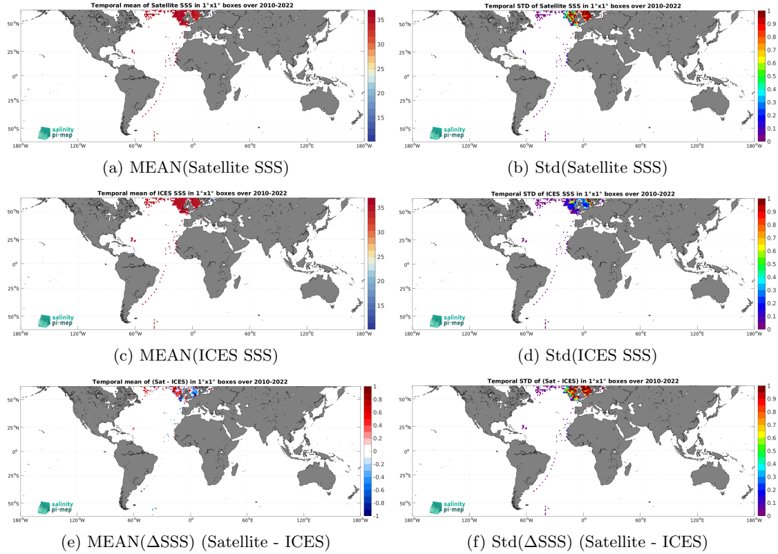
Figure 7: Temporal mean (left) and Std (right) of SSS from SMOS SSS L3 v335 - 10 Days - 25 km (CATDS-CPDC) (top), ICES (middle), and of \Delta SSS (Satellite - ICES). Only match-up pairs are used to generate these maps.
