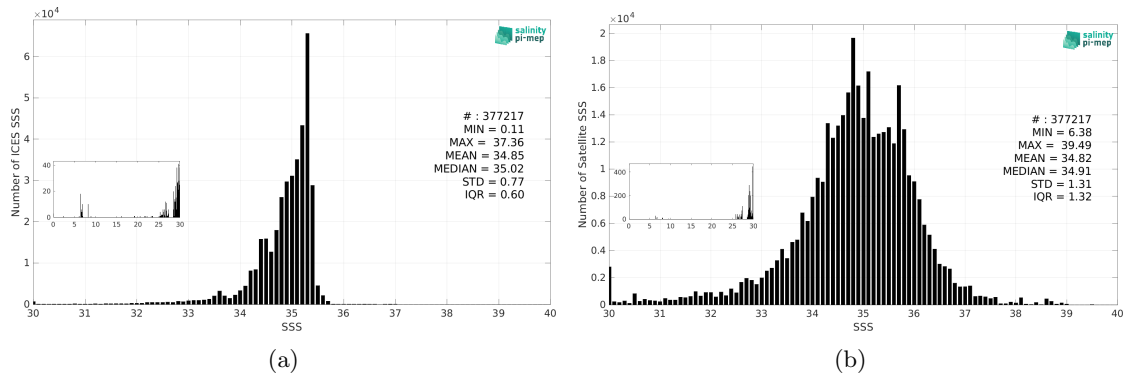
Figure 3: Histograms of SSS from ICES (a) and SMOS SSS L3 v335 - 10 Days - 25 km (CATDS-CPDC) (b) considering all match-up pairs per bins of 0.1 over the SMOS coastal zone (<800km) 60N-60S Pi-MEP region and for the full satellite product period.
