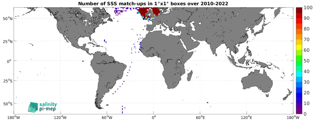
Figure 5: Number of SSS match-ups between ICES SSS and the SMOS SSS L3 v335 - 10 Days - 25 km (CATDS-CPDC) SSS product for the SMOS coastal zone (<800km) 60N-60S Pi-MEP region over 1^\circ \times 1^\circ boxes and for the full satellite product period.
