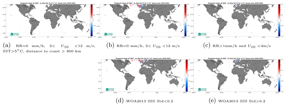
Figure 14: Temporal mean gridded over spatial boxes of size 1^\circ \times 1^\circ of \Delta SSS (SMOS SSS L3 v335 - 10 Days - 25 km (CATDS-CPDC) - ICES) for 5 different subdatasets corresponding to:RR=0 mm/h, 3 < U_{10} < 12 m/s, SST >5^\circ C, distance to coast > 800 km (a), RR=0 mm/h, 3 < U_{10} < 12 m/s (b), RR >1 mm/h and U_{10} < 4 m/s (c), WOA2013 SSS Std <0.2 (d), WOA2013 SSS Std >0.2 (e).
