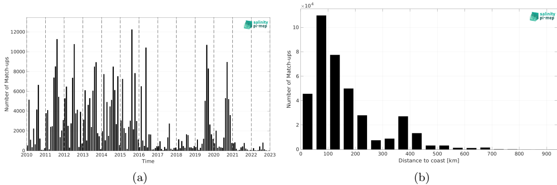
Figure 2: Number of match-ups between ICES and SMOS SSS L3 v335 - 10 Days - 25 km (CATDS-CPDC) SSS as a function of time (a) and as function of the distance to coast (b) over the SMOS coastal zone (<800km) 60N-60S Pi-MEP region and for the full satellite product period.
