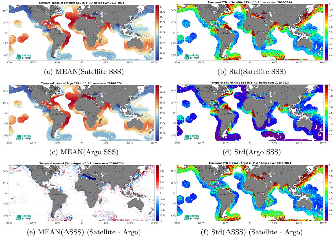
Figure 7: Temporal mean (left) and Std (right) of SSS from SMOS SSS L3 v335 - 10 Days - 25 km (CATDS-CPDC) (top), Argo (middle), and of \Delta SSS (Satellite - Argo). Only match-up pairs are used to generate these maps.
