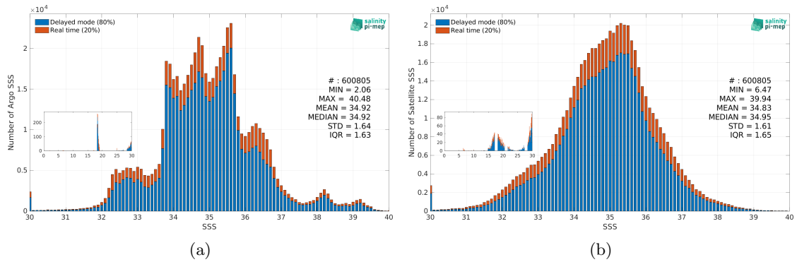
Figure 3: Histograms of SSS from Argo (a) and SMOS SSS L3 v335 - 10 Days - 25 km (CATDS-CPDC) (b) considering all match-up pairs per bins of 0.1 over the SMOS coastal zone (<800km) 60N-60S Pi-MEP region and for the full satellite product period.
