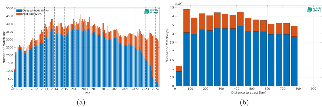
Figure 2: Number of match-ups between Argo and SMOS SSS L3 v335 - 10 Days - 25 km (CATDS-CPDC) SSS as a function of time (a) and as function of the distance to coast (b) over the SMOS coastal zone (<800km) 60N-60S Pi-MEP region and for the full satellite product period.
