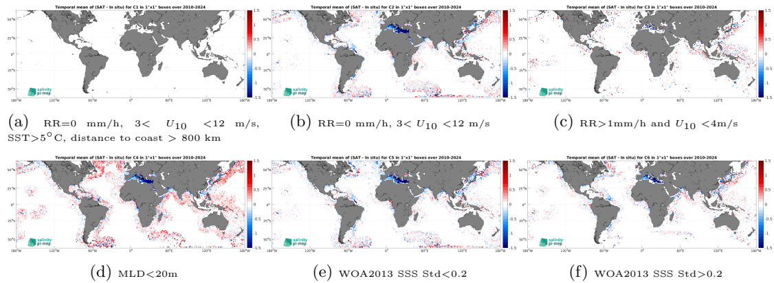
Figure 14: Temporal mean gridded over spatial boxes of size 1^\circ \times 1^\circ of \Delta SSS (SMOS SSS L3 v335 - 10 Days - 25 km (CATDS-CPDC) - Argo) for 6 different subdatasets corresponding to:RR=0 mm/h, 3 < U_{10} < 12 m/s, SST >5^\circ C, distance to coast > 800 km (a), RR=0 mm/h, 3 < U_{10} < 12 m/s (b), RR >1 mm/h and U_{10} < 4 m/s (c),MLD <20 m (d),WOA2013 SSS Std <0.2 (e),WOA2013 SSS Std >0.2 (f).
