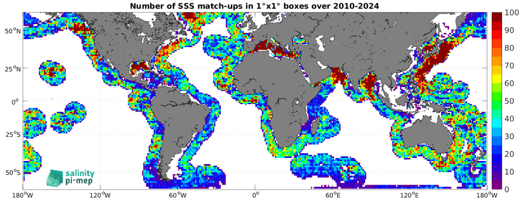
Figure 5: Number of SSS match-ups between Argo SSS and the SMOS SSS L3 v335 - 10 Days - 25 km (CATDS-CPDC) SSS product for the SMOS coastal zone (<800km) 60N-60S Pi-MEP region over 1^\circ \times 1^\circ boxes and for the full satellite product period.
