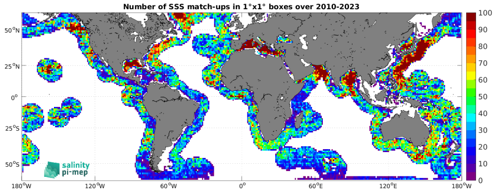
Figure 4: Number of SSS match-ups between Argo SSS and the SMOS SSS L3 v335 - 10 Days - 25 km (CATDS-CPDC) SSS product for the SMOS coastal zone (<800km) 60N-60S Pi-MEP region over 1^{\circ} \times 1^{\circ} boxes and for the full satellite product period.
